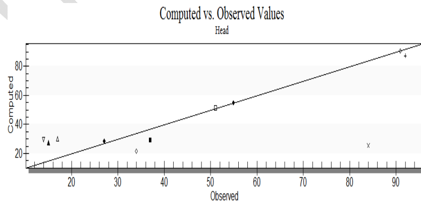
Fig. 4. Ratio 1:1 Line of Computed and Observed Heads for the Model Domain
