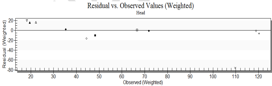
Fig. 7. Plot of Weighted Residual versus Observed Values for the Model Domain
