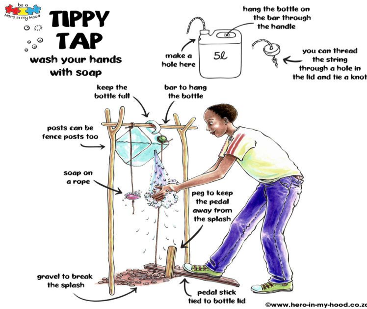
Figure 3: Tippy Tap devices
