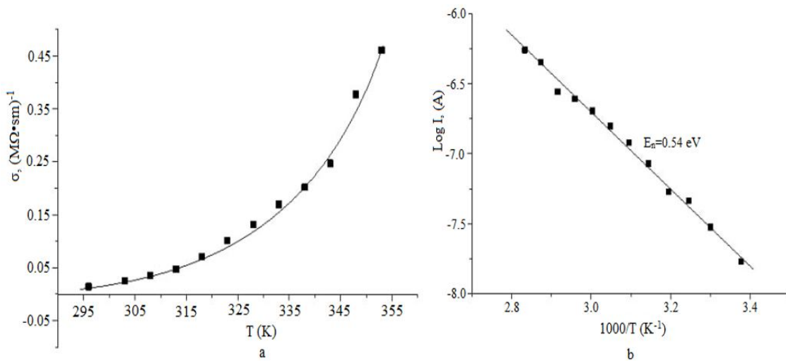
Pic No 4. Temperature dependence of electrical conductivity \sigma of a sample of "Xorazm-150" grade CF KMnO_4 -doped at t=80^\circ C for 7 hours (a) and Arrhenius diagram of this result (b)
