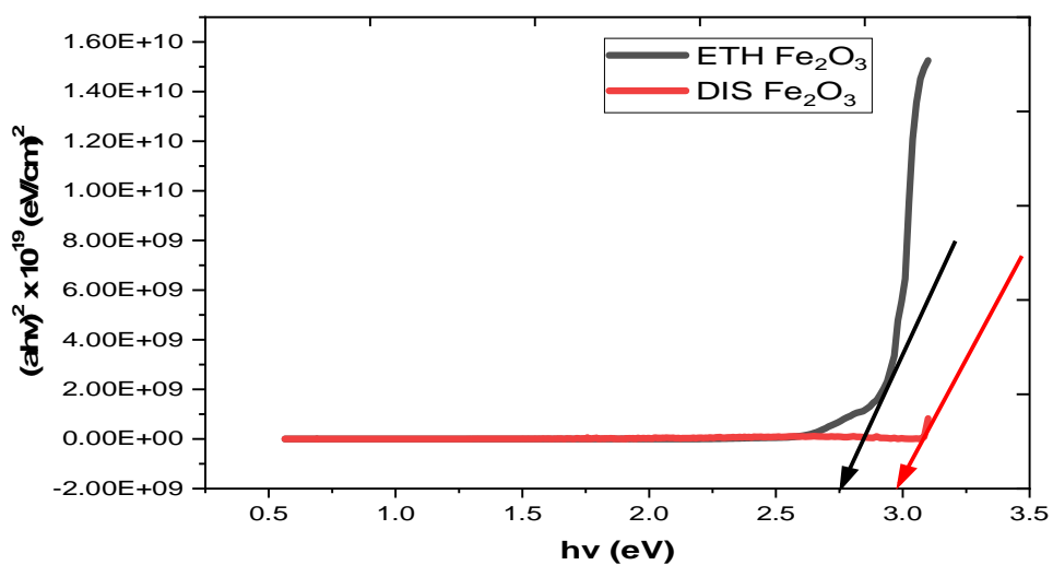
Fig. 3.5: Optical energy bandgap plots of Fe 2 O 3 nanoparticles
