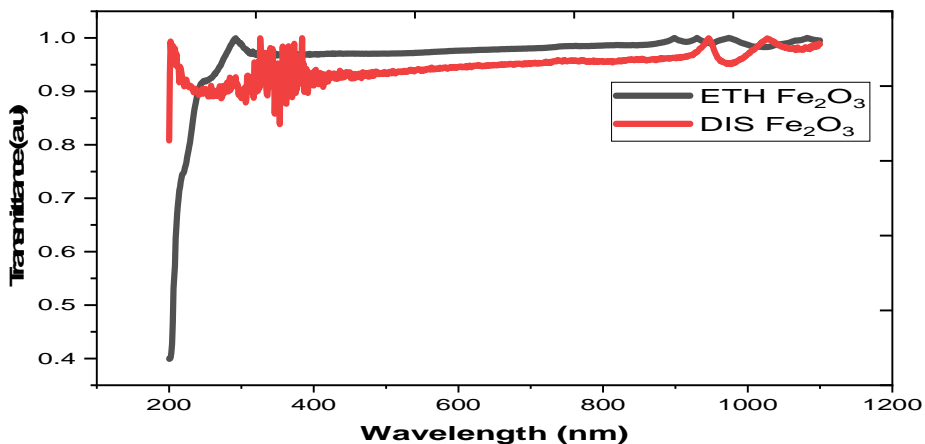
Figure 3.3: Transmittance spectra of \text{Fe}_2\text{O}_3 nanoparticles
