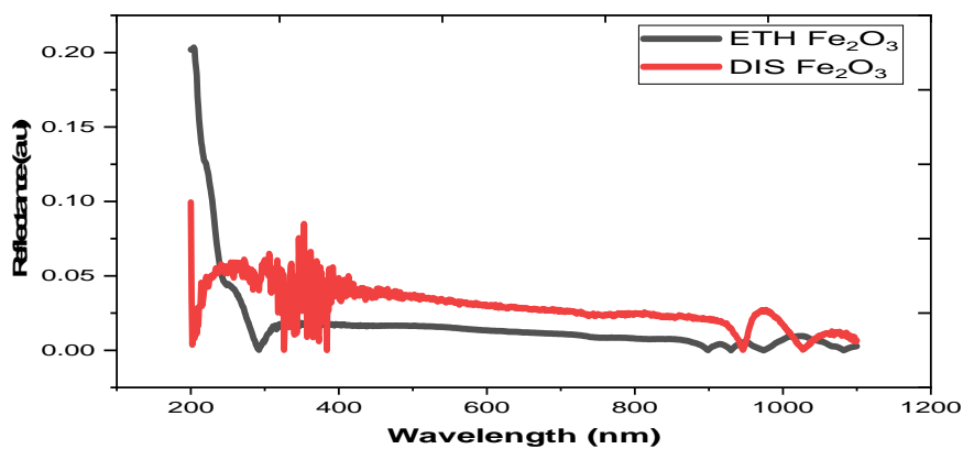
Figure 3.4: Reflectance spectra of Fe_2O_3 nanoparticles
