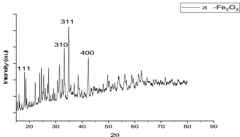
Figure 3.1 X-ray diffractive analysis for \text{Fe}_2\text{O}_3
