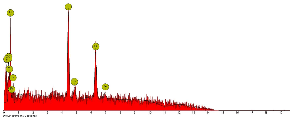
Figure 3 EDX spectrum of iron oxide nanoparticles prepared by a ball milling machine
