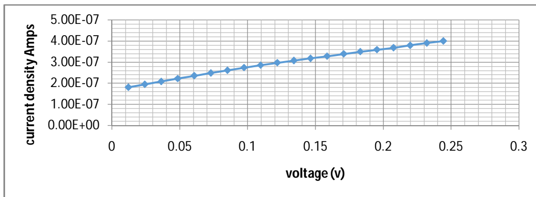
Figure 3.7 I-V characteristic of \text{Fe}_2\text{O}_3 nanoparticles
