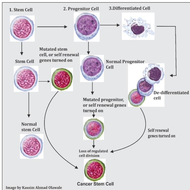
Figure 2: Adapted schematic illustrating carcinogenesis, arising from stem cells, progenitor cells and differentiated cells.
