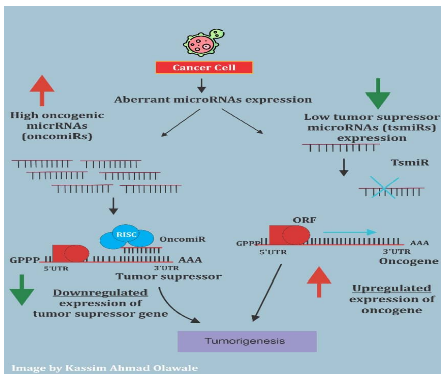
Figure 3: Adapted illustration showing the microRNAs Regulatory roles in BCSCs and tumorigenesis.
