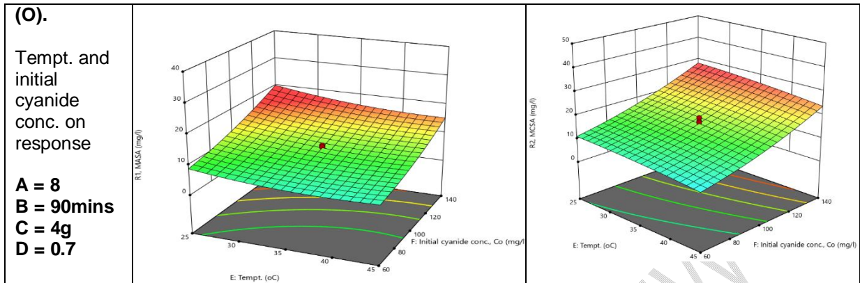
Fig. 6: 3D interaction between the adsorption parameters on R1 and the corresponding R2.
