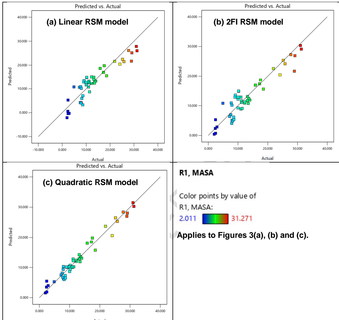
Fig. 3: Design Expert software plot of actual values versus predicted values for R1 of all three RSM models studied
