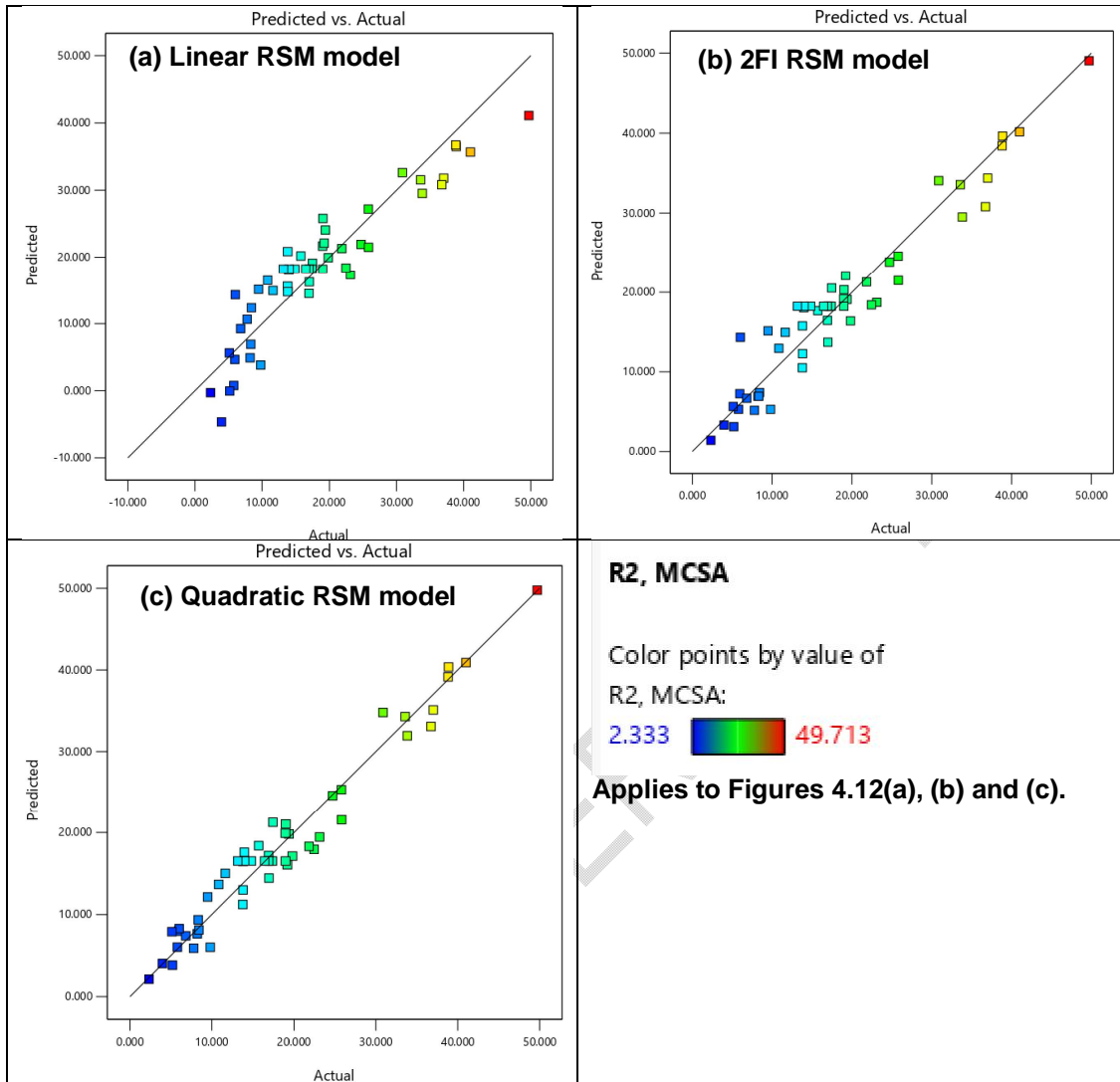
Fig. 5: Design Expert software plot of actual values versus predicted values for R 2 of all three RSM models studied
