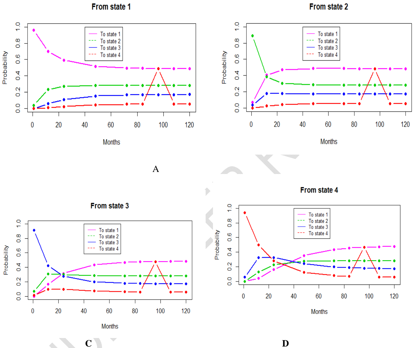
Fig. 2. Conditional probabilities for each state
