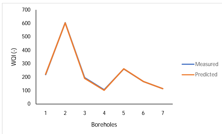
Figure 9: Measured and predicted WQI
