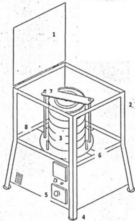
Fig. 2. Design and assembly of the mechanical sieve shaker
