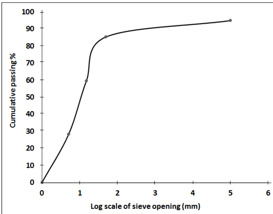
Fig. 4. Grading Curve.
