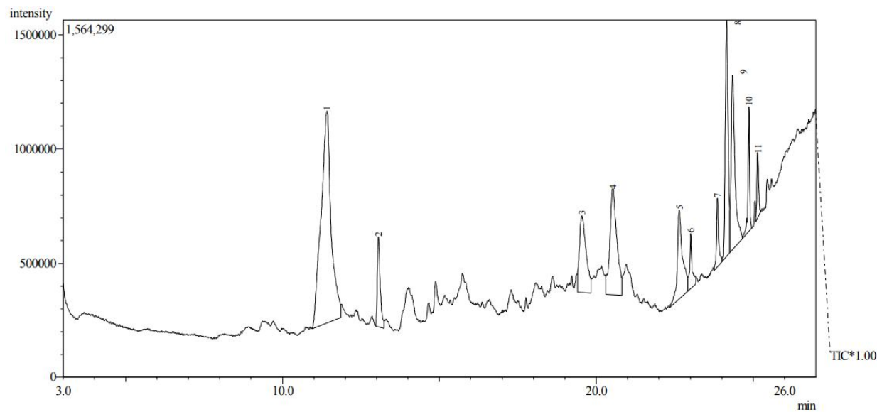
Fig.4. GC-MS chromatogram of LME 6 fraction of H. madagascariensis .
