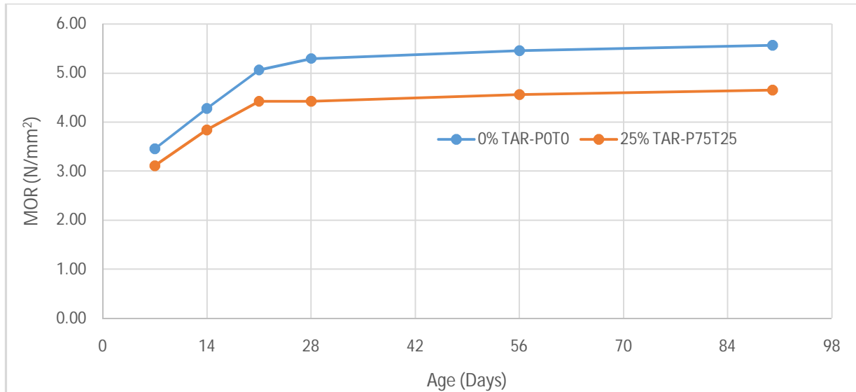
Fig. 5- Modulus of Rupture with age of curing
