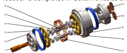
Fig.1.RV reducer parts explosion diagram
