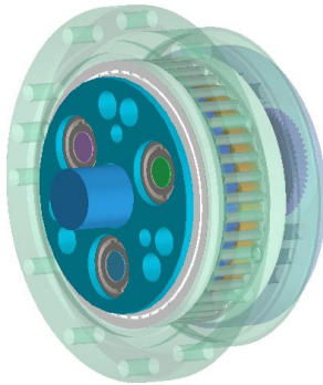
Fig.2. RV reducer interference test
