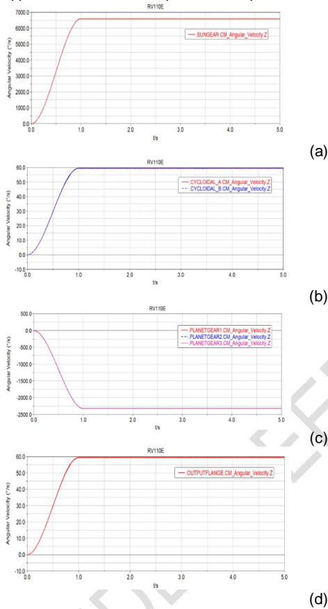
Fig.4.Speed curve of each part
