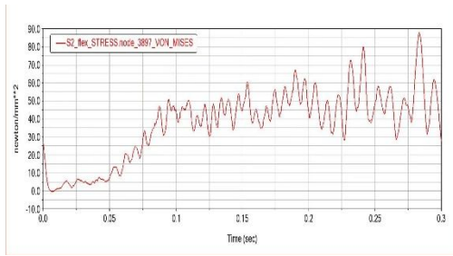
Fig. 5. Time domain diagram of contact stress of needle roller bearing
