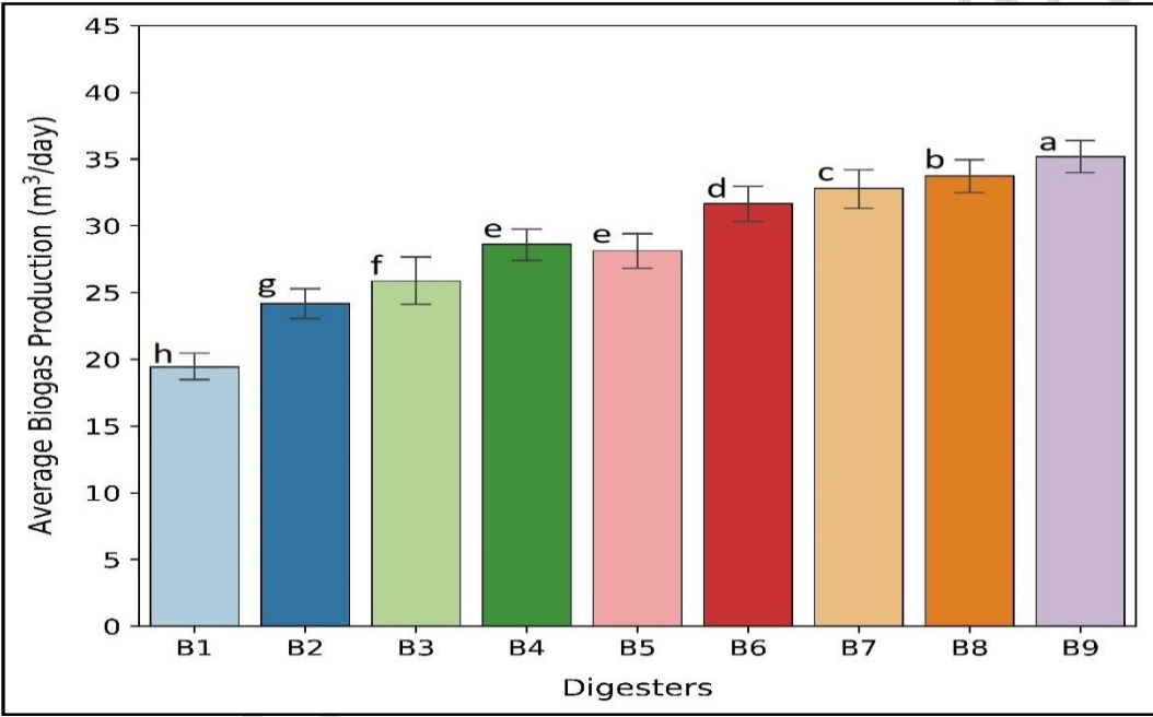
Figure 2: Average Production volume of biogas in the different digesters
