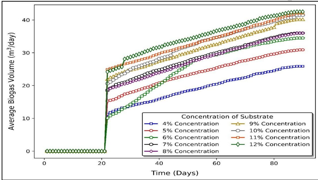
Figure 1: Production of biogas in the nine digesters over a period of 90 days
