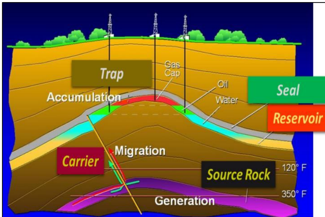
Figure 1. A sedimentary basin showing the five elements of a petroleum systems which includes reservoir (Craig and Quagliaroli, 2020)
