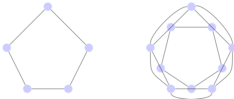
Figure 3: C_5 graph and its total graph T(C_5)
