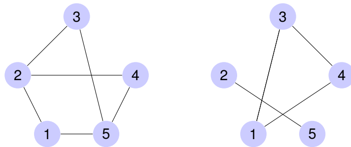
Figure 1: A Graph and its complement
