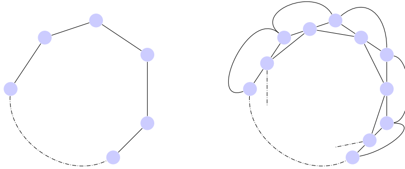
Figure 5: C_n graph and the corresponding total graph T(C_n)
