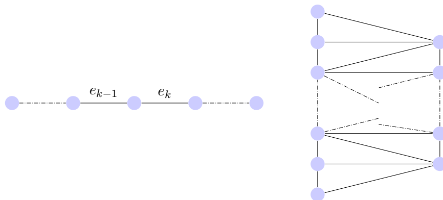
Figure 4: P_n graph and the corresponding total graph T(P_n)
