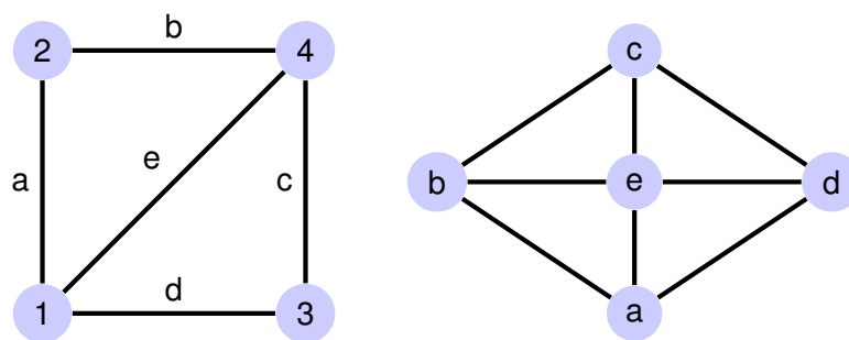
Figure 2: A Graph G and the corresponding line graph L(G)
