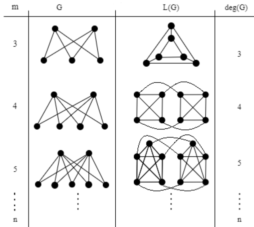
Figure 6: Bipartite graph and corresponding line graph for fix n = 2
