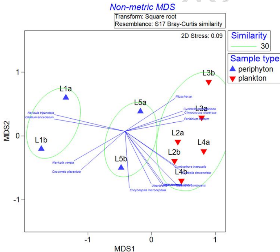
Fig.2. Non-metric multidimensional scaling (nMDS) overlaid with clusters of group average clustering (30% of similarity) of locations based on Bray-Curtis matrix of
