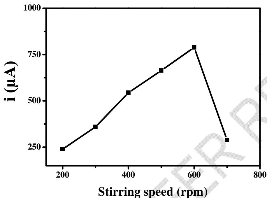
Fig. 10. Effect of mechanical stirring speed on peak current intensity by DPASV. [\text{Hg}^{2+}] 35\mu\text{M} ; scan rate 20\text{ mV/s} ; deposition time 120\text{ s} ; pulse amplitude 50\text{ mV}
