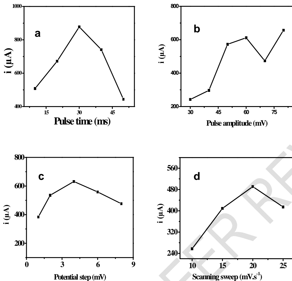
Fig. 11. Influence of DPV parameters (a. Pulse time; b. Pulse amplitude; c. Potential step; and d. Scanning sweep) on the peak current intensity by DPASV for determination of 35 \mu\text{M Hg}^{2+} in 0.8 \text{ M HClO}_4
