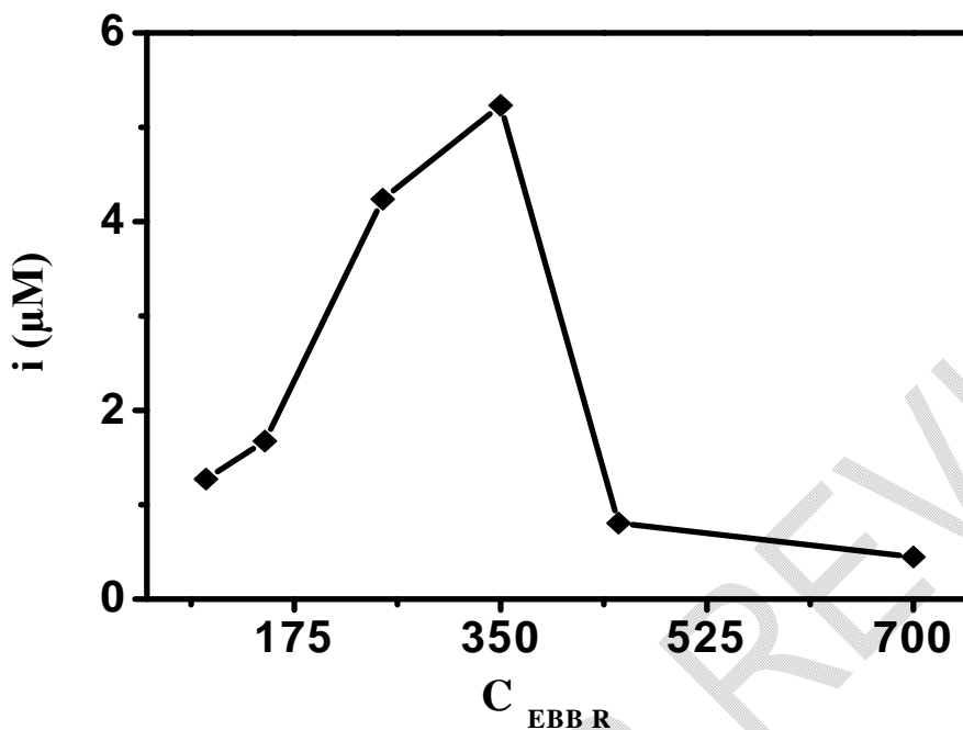
Fig. 5. Effect of the variation of the EBB R (Calcon) concentration on the peak current intensity by DPASV. [ \text{Hg}^{2+} ] 35 \mu\text{M} ; scanning speed 20 mV/s; deposition time 120 s; pulse amplitude 50 mV
