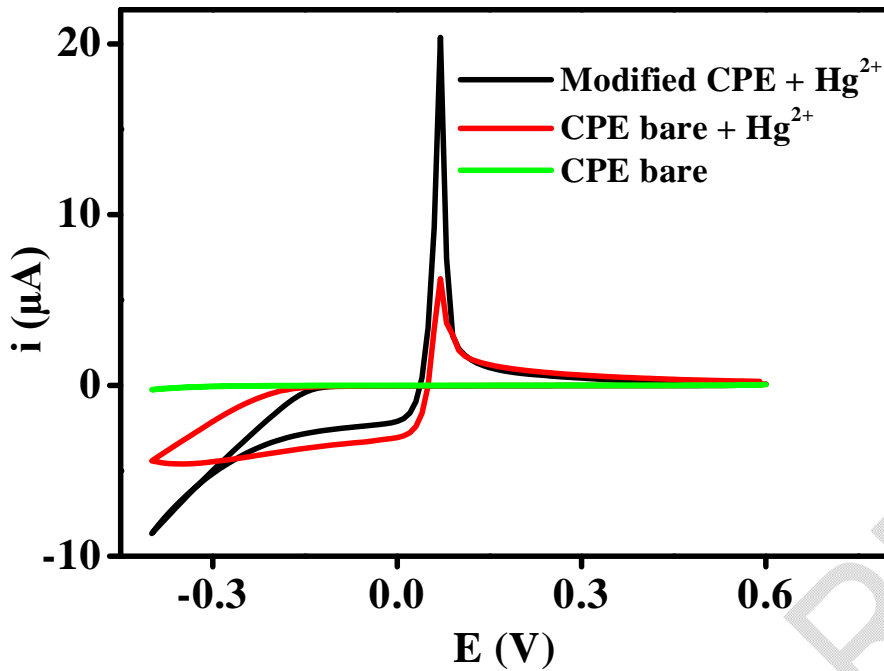
Fig. 3. Cyclic voltammograms obtained at: a. bare CPE, b. bare CPE containing 2.5 \cdot 10^{-4} M \text{Hg}^{2+} and c. poly(EBB R)-CPE containing 2.5 \cdot 10^{-4} M \text{Hg}^{2+} in 1 M KCl; Scan rate 50 mV/s
