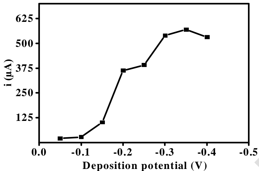
Fig. 8. Effect of the variation of the deposition potential on the peak current intensity by DPASV. [\text{Hg}^{2+}] 35 \mu\text{M} ; scan rate 20 mV/s; pulse amplitude 50 mV; stirring speed 400 rpm
