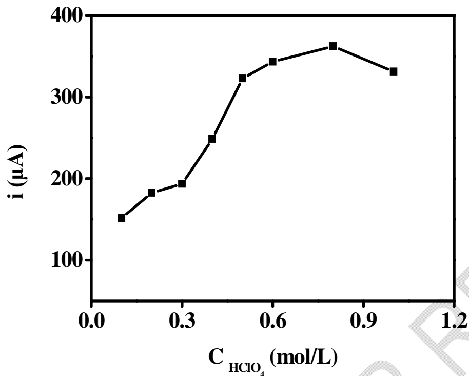
Fig. 7. Effect of concentration of \text{HClO}_4 on DPASV peak current for the determination of 35\mu\text{M Hg}^{2+} [can you show the error bars on this and the other figures?]
