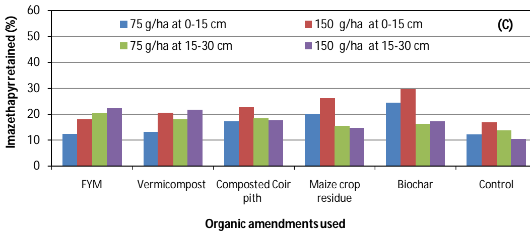
Fig 1. Effect of different organic amendments and rates of herbicides application on their retention percent in soil at different depths (A. pendimethalin; B. Atrazine; C. Imazethapyr)
