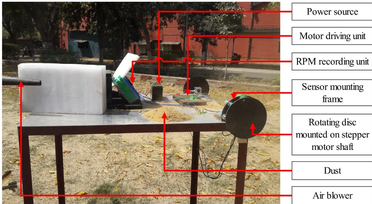
Figure 1. Experimental setup in outdoor dusty condition
