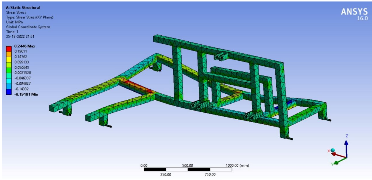
Fig.4: Maximum shear stress on the frame Equivalent stress (Von Mises)
