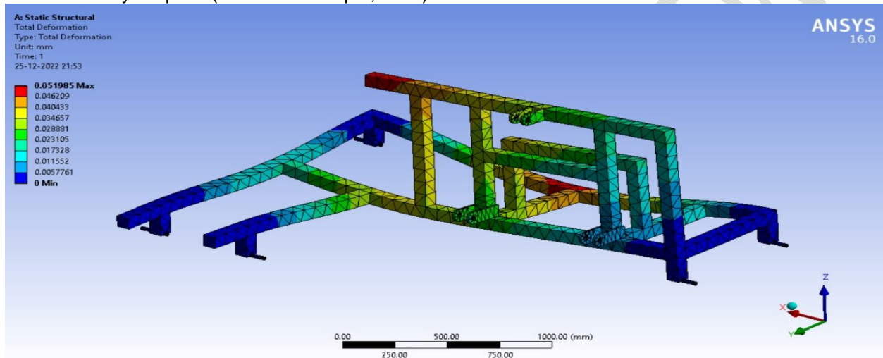
Fig. 3: Total deformation on frame Maximum Shear Stress
