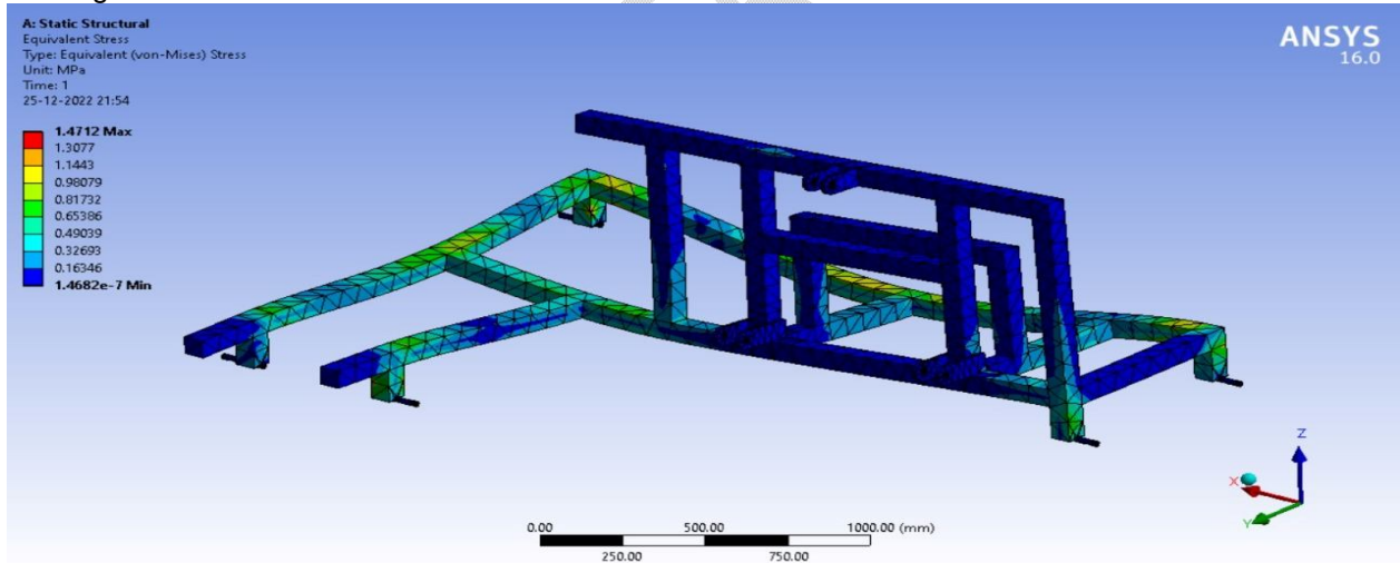
Fig. 5: Equivalent von-mises stress on the frame 4. CONCLUSION
