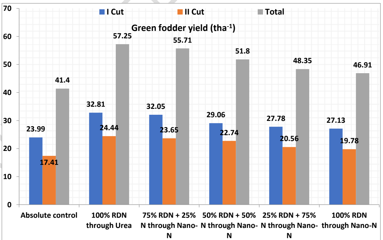
Fig. 2: Effect on different nitrogen treatments on green fodder yield of oats
