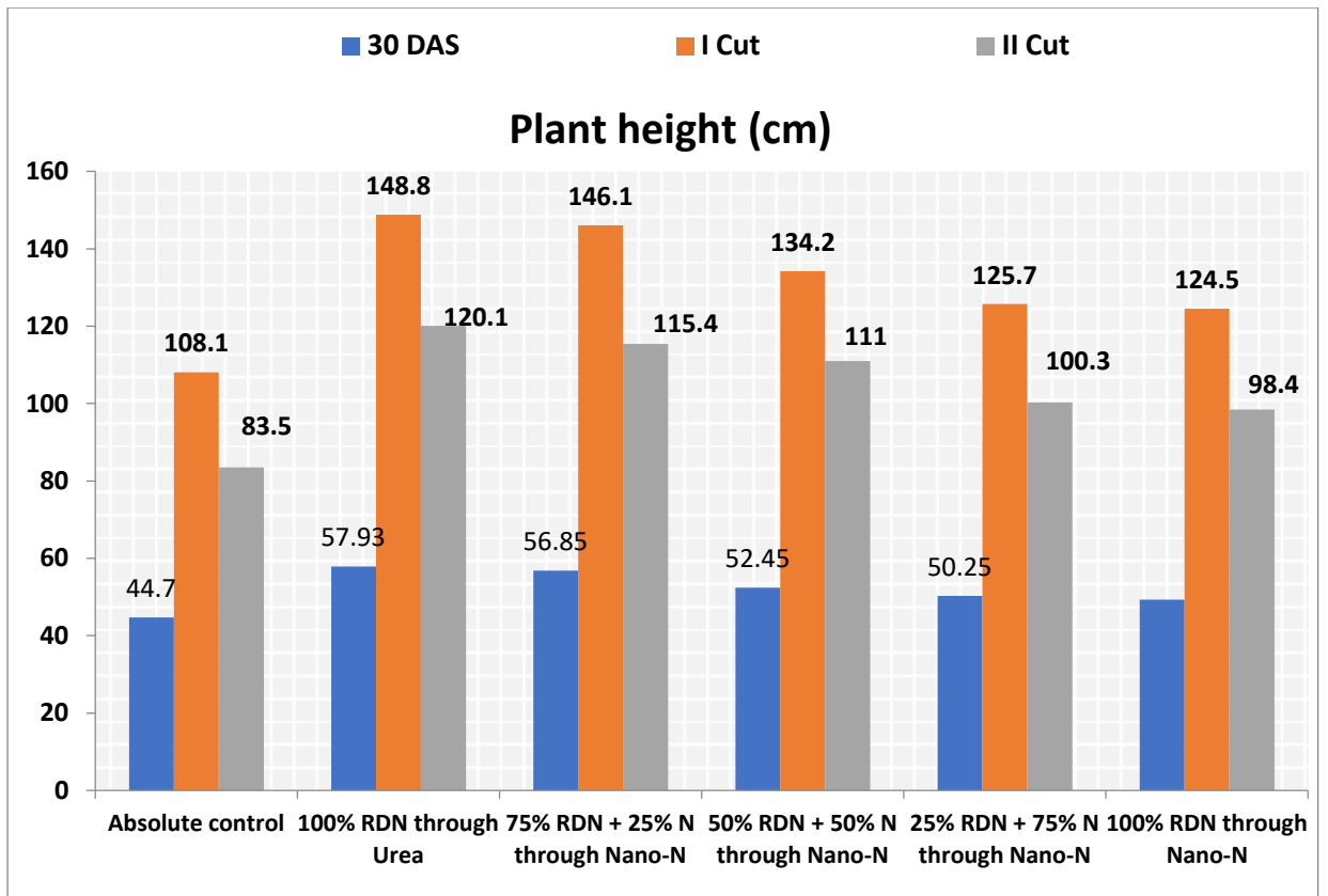
Fig. 1: Effect on different nitrogen treatments on plant height of oats
