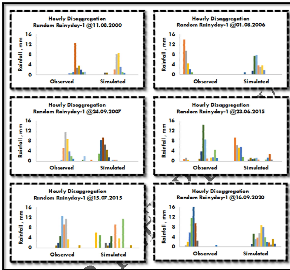
Fig. 4 Predictive performance of BLRPM used with its location specific parameters for randomly opted rainy days (6 nos) for a sample study location (Dakor)
