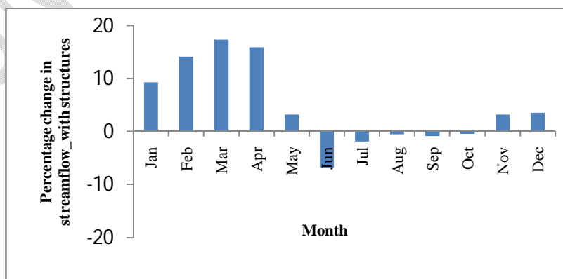
Fig. 5 Percentage change in streamflow due to the addition of structures
