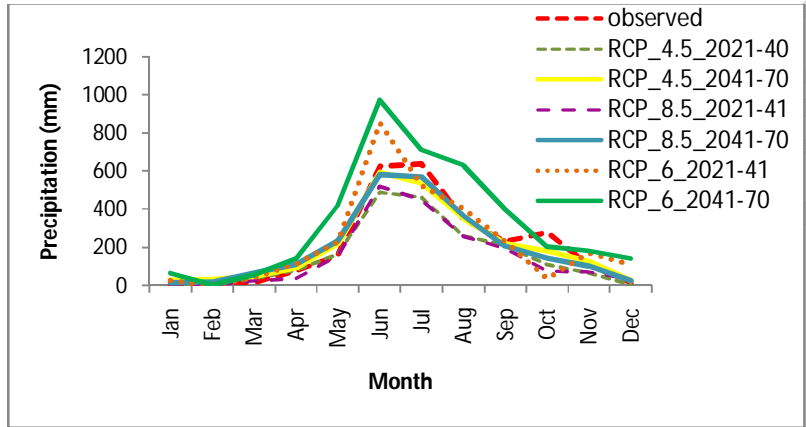
Fig. 6 Comparison of observed and bias corrected monthly precipitation under different scenarios
