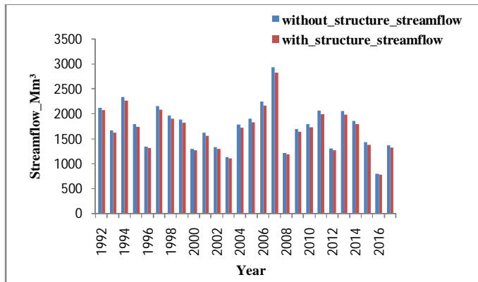
Fig. 3 Predicted annual streamflow simulation with and without conservation structures
