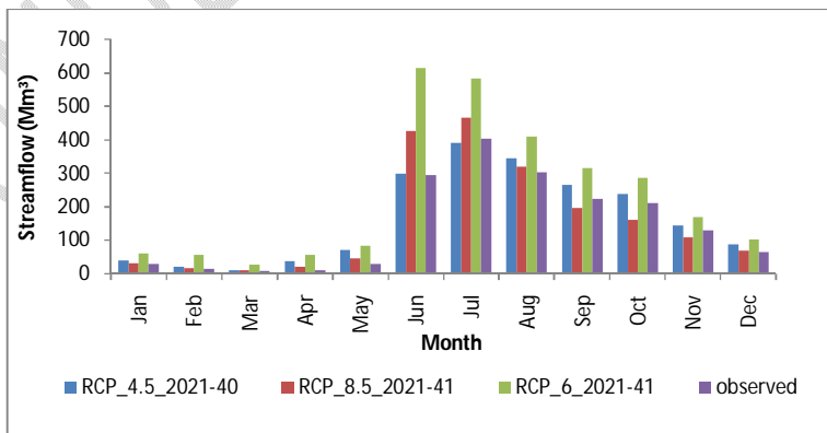
Fig. 12 Predicted monthly streamflow under different scenario from 2021-40
