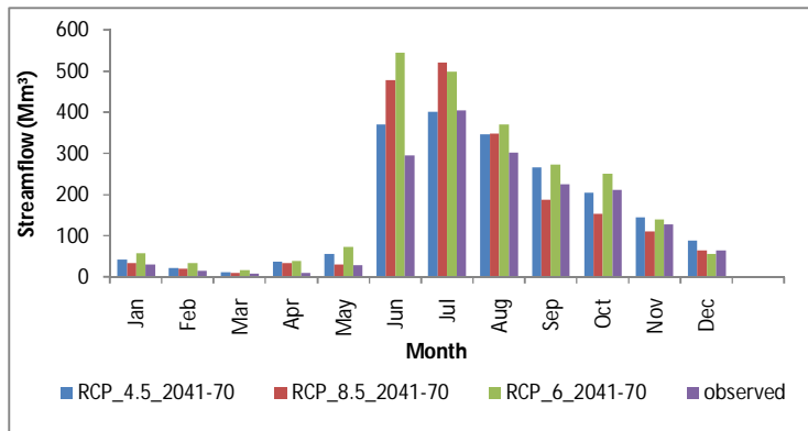
Fig. 13 Predicted monthly streamflow under different scenario from 2041-70
