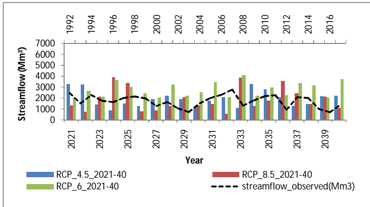
Fig. 10 Predicted annual streamflow under different scenario from 2021-40
