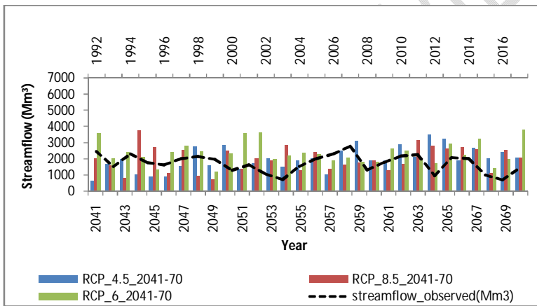
Fig. 11 Predicted annual streamflow under different scenario from 2041-70
