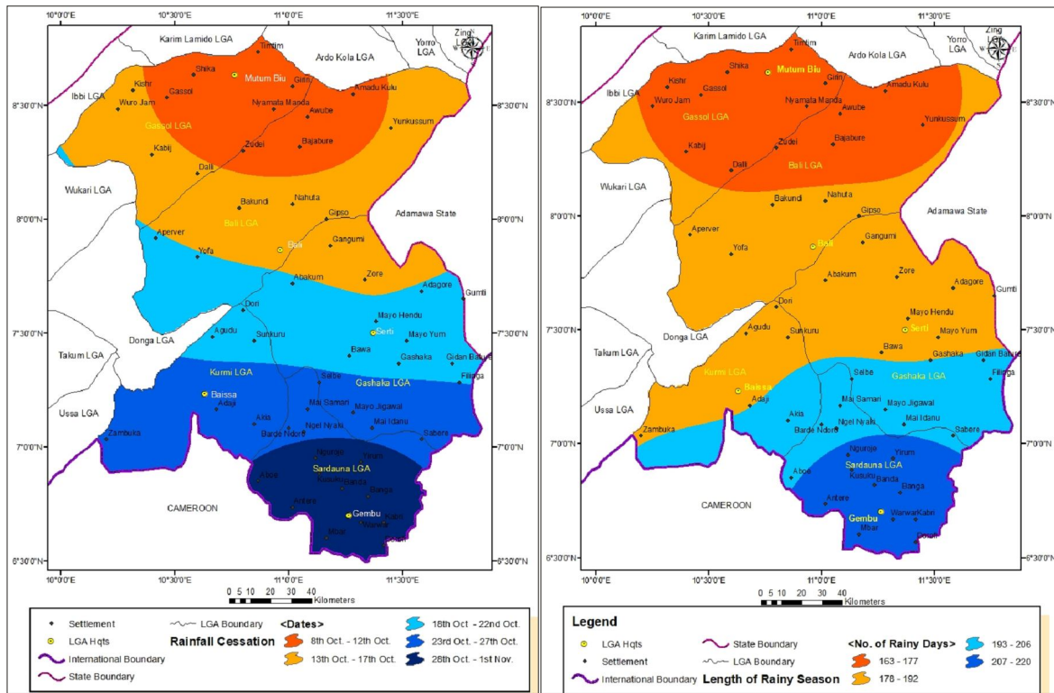
Figure 2c. Spatial pattern of rainfall cessation. Figure 2d. Spatial pattern of length of rainfall
