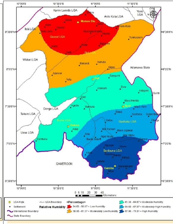
Figure 4b. Mean annual relative humidity
