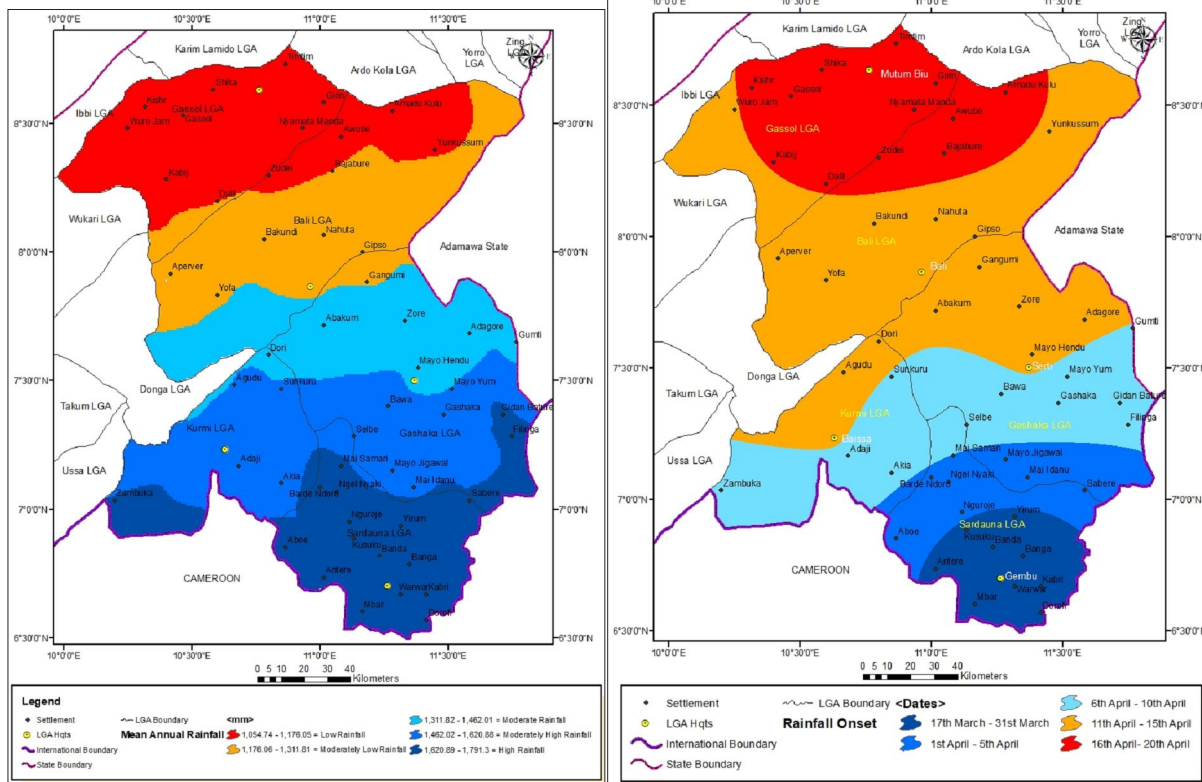
Figure 2a. Spatial pattern of mean annual rainfall. Figure 2b. Spatial pattern of rainfall Onset
