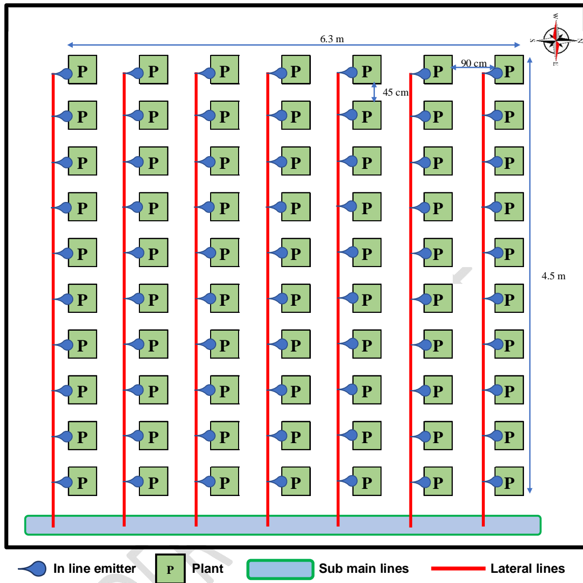
Figure 2. Singleplot layout
