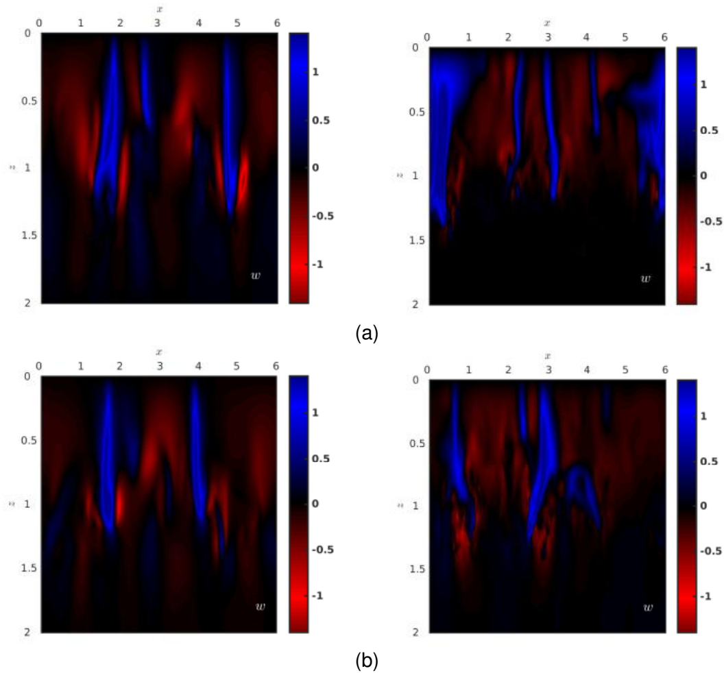
Figure 9: The vertical velocity field at computational times (a) t \approx 26 and (b) t \approx 35 for the case \sigma = 0.1 in two-dimensions (left) and three-dimensions (right).
