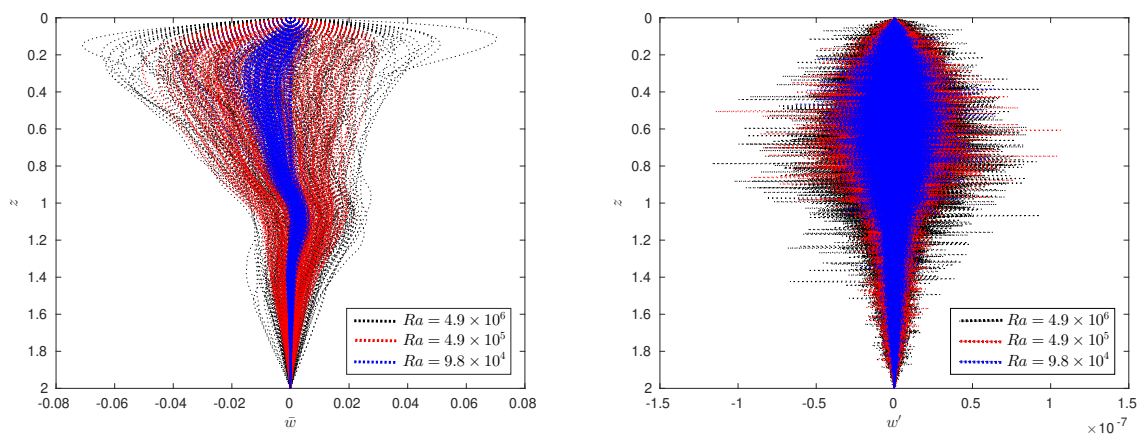
Figure 3: Temporal line graphs of the average component (left panel) and fluctuating component (right panel) of the w -velocity field for several Ra values.
