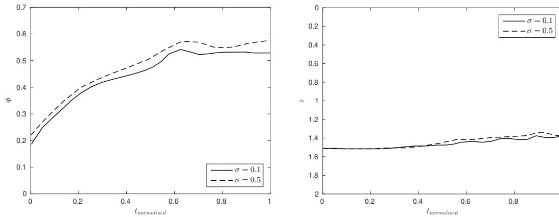
Figure 14: The temporal evolution of the magnetic flux fraction contained above the initial location of magnetic field, \Phi , (left panel) and the location of the maximum magnetic field, z_{max} (right panel).
