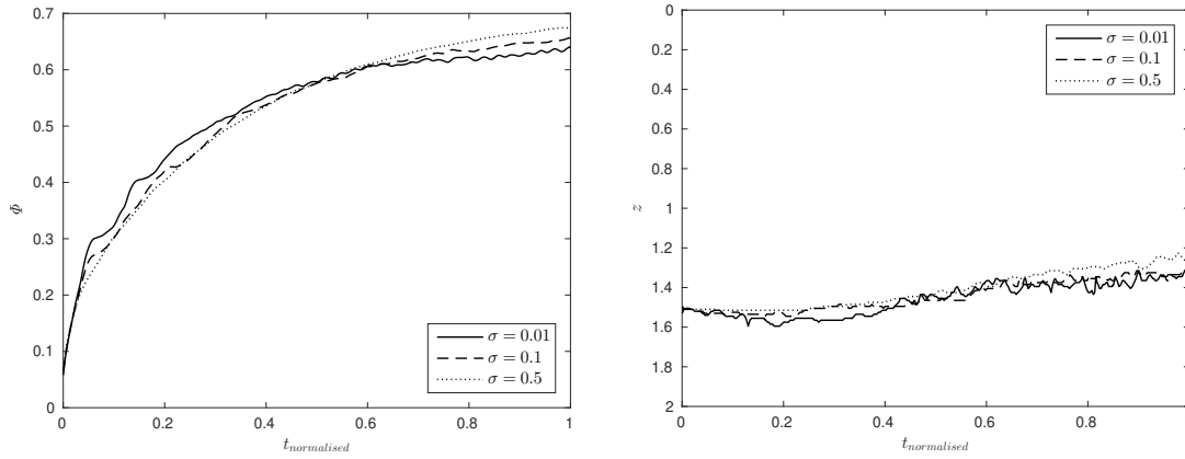
Figure 8: The temporal evolution of the magnetic flux fraction contained above the initial location of magnetic field, \Phi , (left panel) and the location of the maximum magnetic field, z_{max} (right panel).
