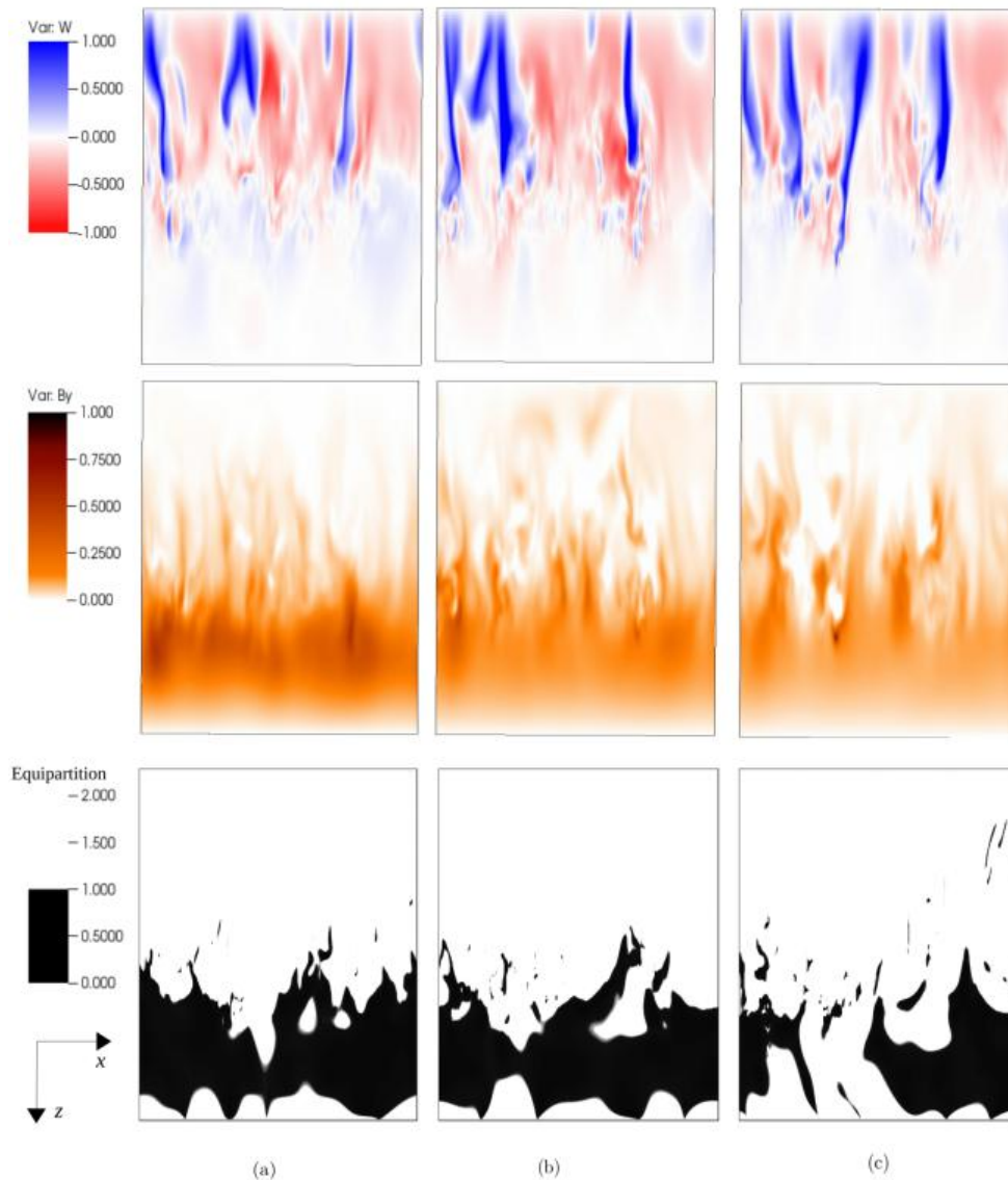
Figure 13: Snapshots of the z -component of the velocity field (top), the y -component of the magnetic field (middle) and ratio of the kinetic to magnetic energy (bottom) at y = 0 for times (a) t = 45.3 , (b) t = 50.9 , and (c) t = 55.6 respectively.
