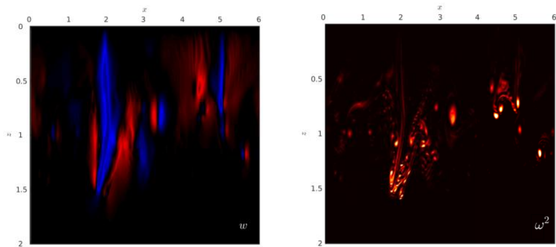
Figure 2: Snapshots of the vertical velocity field (left panel) and enstrophy (right panel) for \sigma = 0.01 at a statistically steady state. The colours red and blue in the velocity field correspond to upward and downward convective motions respectively. Strong enstrophy densities are yellow, whereas weaker densities are dark and translucent.
