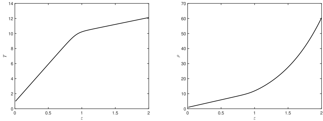
Figure 1: Initial background states of temperature (left panel) and density (right panel) for d = 2 , T_0 = 1 , \rho_0 = 1 , \theta = 10 with m_T = 1 and m_B = 9 .
