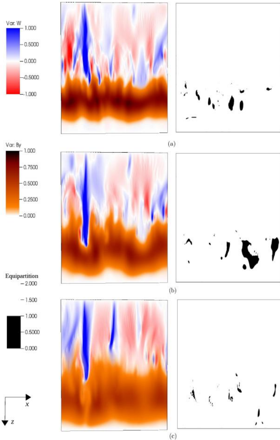
Figure 5: Snapshots of the the z -component of the velocity field overlaid with the y -component of the magnetic field (left) and ratio of the kinetic to magnetic energy (right) at (a) t = 40.68 , (b) t = 41.21 , and (c) t = 42.03 respectively.
