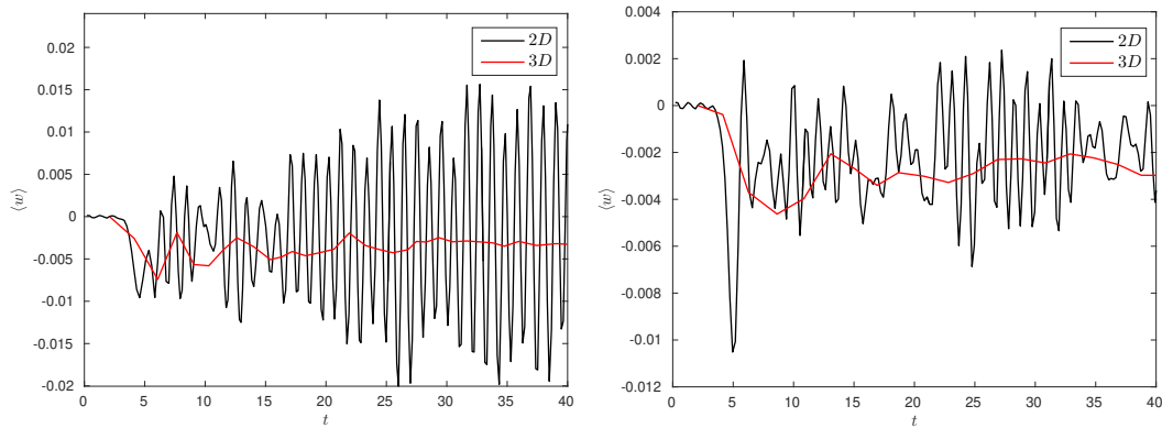
Figure 10: Temporal evolution of the average vertical velocity for \sigma = 0.1 (left panel) and \sigma = 0.5 (right panel) in two- and three-dimensions.
