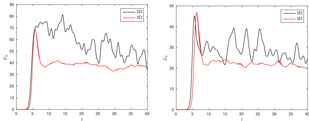
Figure 11: Temporal evolution of the total kinetic energy for \sigma = 0.1 (left panel) and \sigma = 0.5 (right panel) in two- and three-dimensions.
