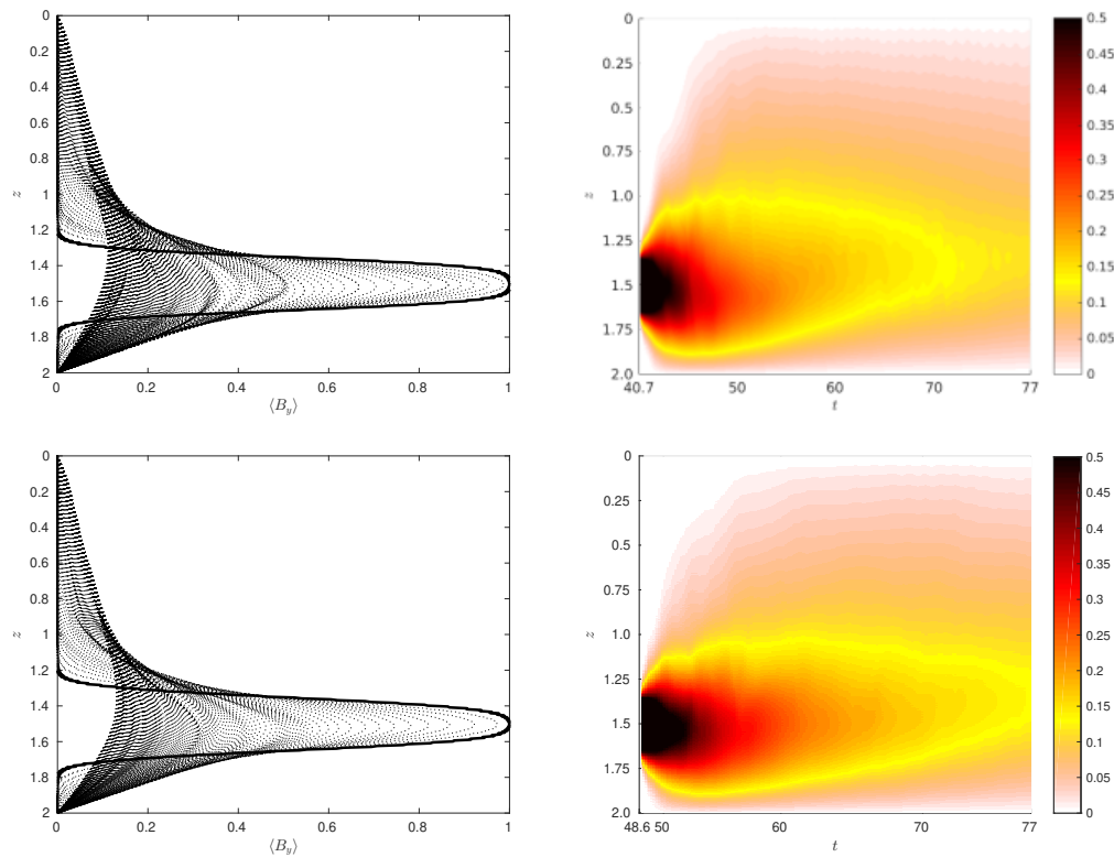
Figure 7: Line graphs (left) and colour spacetime diagrams (right) of the horizontal average of the magnetic field in the y -direction, B_y for \sigma = 0.01 (top panel) and \sigma = 0.1 (bottom panel), where F = 0.01 .
