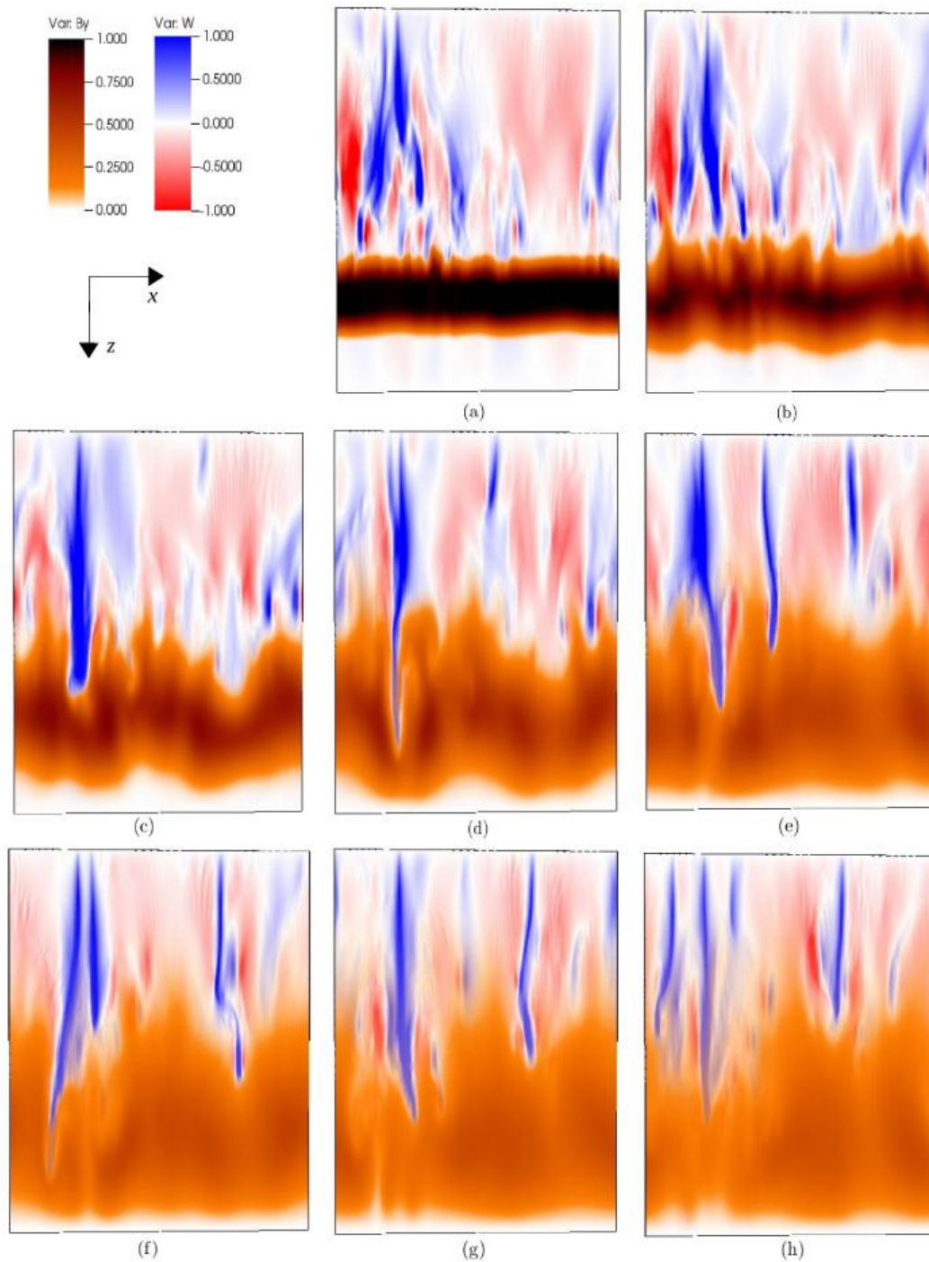
Figure 4: Snapshots of the z -component of the velocity field overlaid with the y -component of the magnetic field at computational times (a) t = 40.68 , (b) t = 41.21 , (c) t = 42.03 , (d) t = 43.04 , (e) t = 44.50 , (f) t = 45.73 , (g) t = 46.87 , and (h) t = 47.92 respectively.
