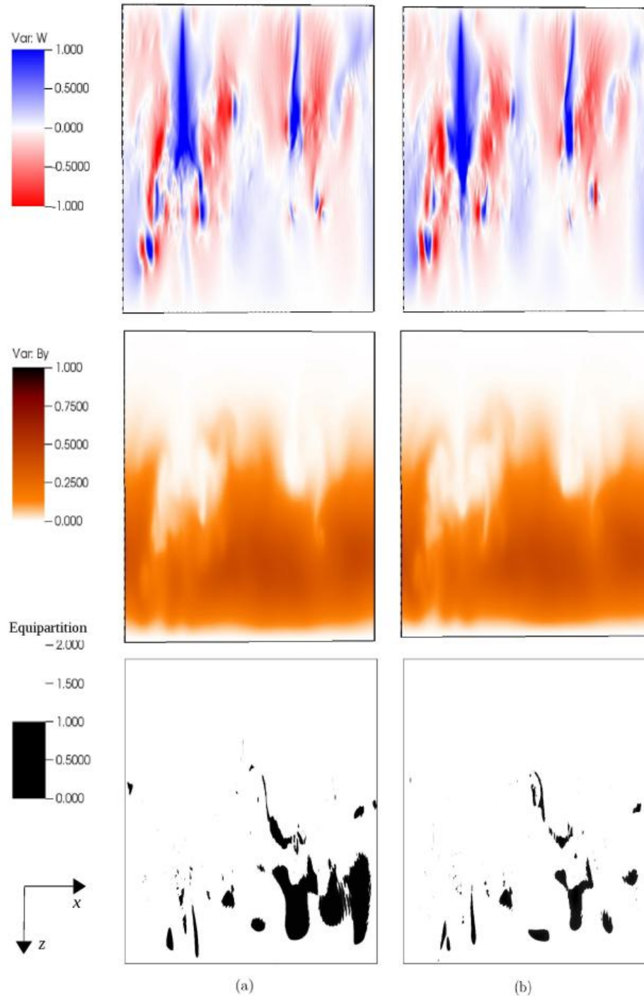
Figure 6: Snapshots of the z -component of the velocity field (top), the y -component of the magnetic field (middle) and ratio of the kinetic to magnetic energy (bottom) at (a) t = 46.31 and (b) t = 46.56 respectively.
