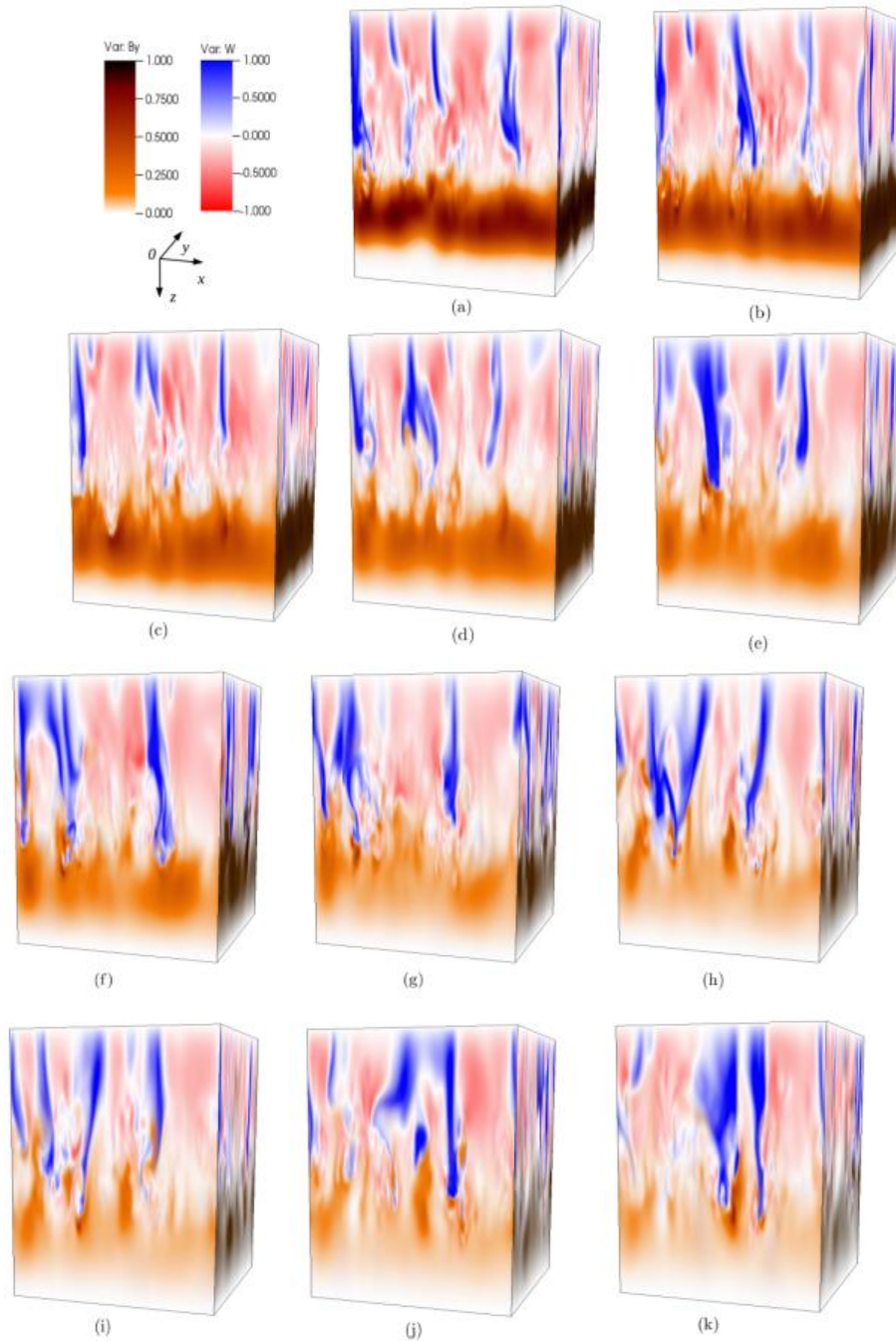
Figure 12: Snapshots of the z -component of the velocity field overlaid with the y -component of the magnetic field in three-dimensions at computational times (a) t = 41.78 , (b) t = 43.02 , (c) t = 44.15 , (d) t = 46.40 , (e) t = 48.60 , (f) t = 49.80 , (g) t = 52.16 , (h) t = 54.66 , (i) t = 55.61 , (j) t = 57.37 and (k) t = 58.69 respectively.
