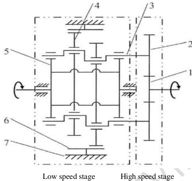
Figure 2 RV transmission mechanism diagram
