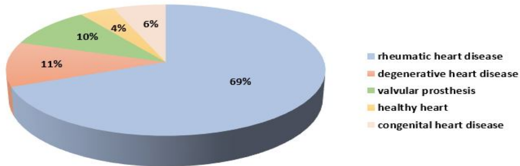
Figure 1: Distribution of heart disease underlying infective endocarditis
