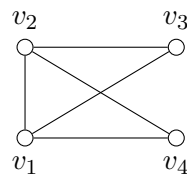
Figure 2: The graph G
