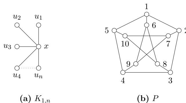
Figure 1: The Star graph K_{1,n} and the Petersen graph P
