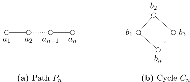
Figure 3: The path P_n and the cycle C_n
