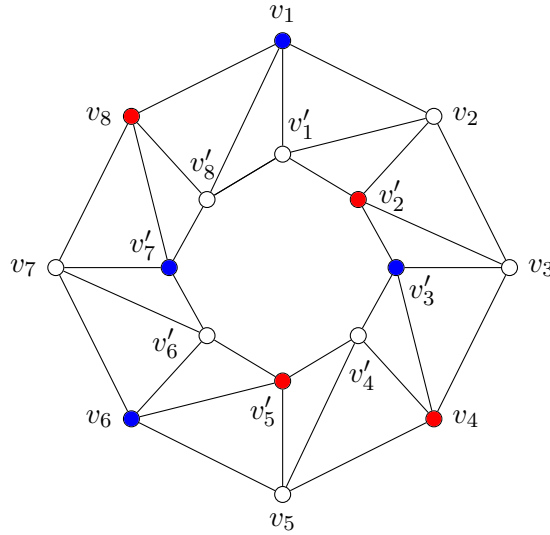
Figure 5: The minimum rings dominating sets in T(C_8)
