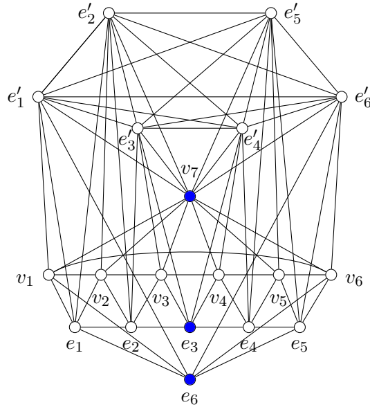
Figure 9: The minimum rings dominating set in T(W_6)
