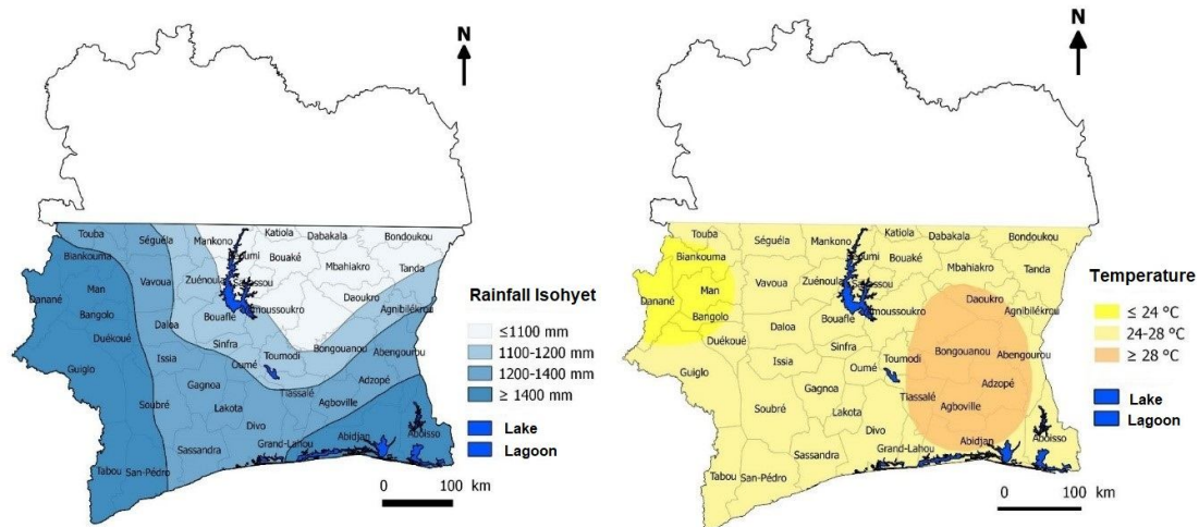
Figure 1: Rainfall and temperature maps
