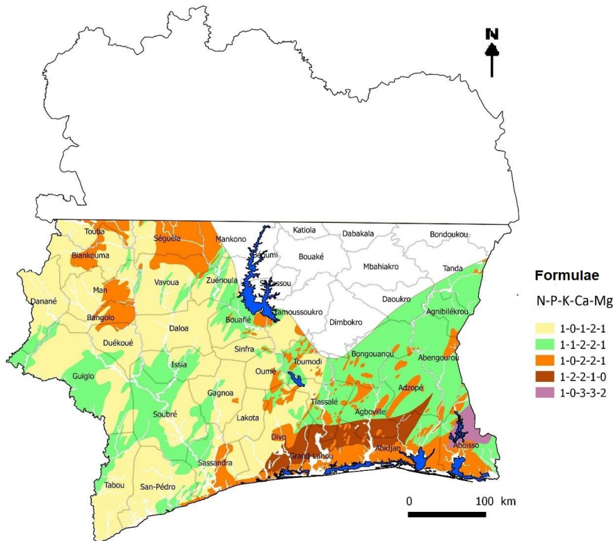
Figure 5: Nutrient requirement maps for mature coffee trees in Côte d'Ivoire
