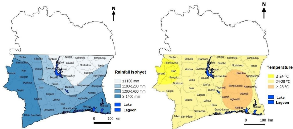
Figure 1: Rainfall and temperature maps
