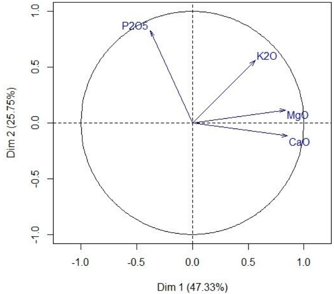
Figure 2: Representation of the variables (chemical needs) in the (1;2) factorial plane
