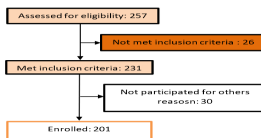
Fig. 1. Sample population
