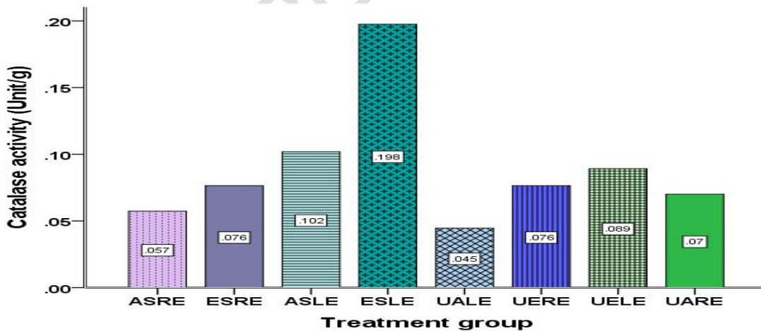
Figure 9: Catalase activity (unit/g) of soaked and unsoaked aqueous and ethanolic extracts Petiveria alliacea leaf and root
