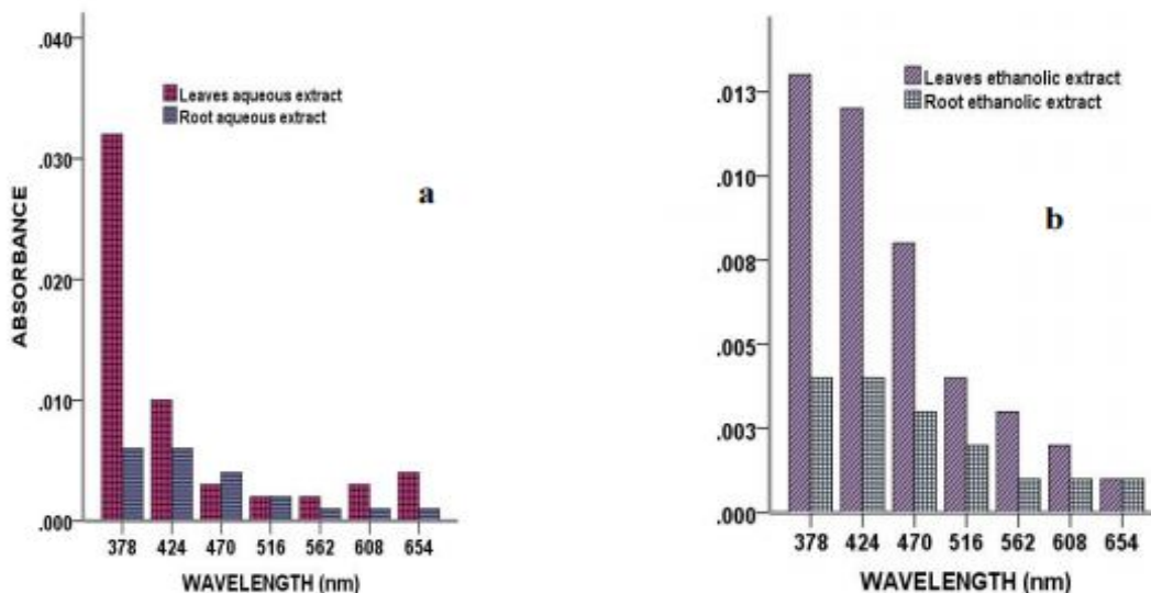
Figure 2: UV-Visible spectrophotometric profile of 0.025g/ml aqueous (a), and ethanolic (b) extracts of Petiveria alliacea leaves and root
