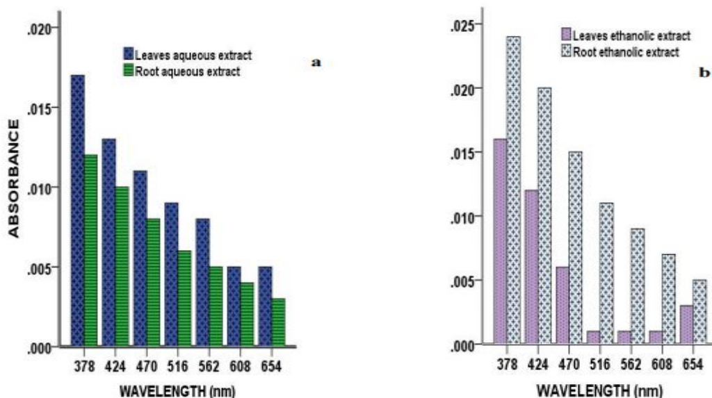
Figure 1: UV-Visible spectrophotometric profile of 0.01g/ml aqueous (a), and ethanolic (b) extracts of Petiveria alliacea leaf and root
