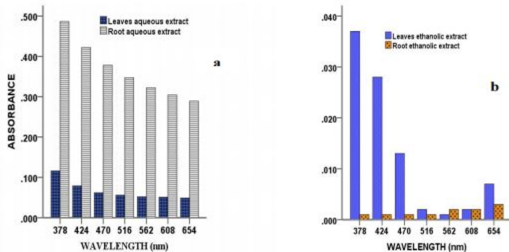
Figure 5: UV-Visible spectrophotometric profile of 0.15g/ml aqueous (a), and ethanolic (b) extracts of Petiveria alliacea leaf and root
