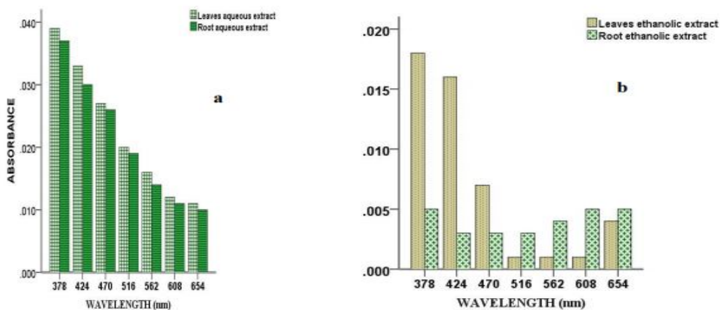
Figure 3: UV-Visible spectrophotometric profile of 0.075g/ml aqueous (a), and ethanolic (b) extracts of Petiveria alliacea leaf and root
