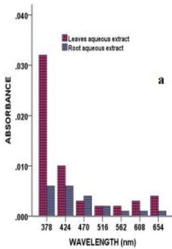
Figure 2:- UV-Visible spectrophotometric profile of 0.025g/ml aqueous (a) and ethanolic (b) extracts of Petiveriaalliacea leaves and root
