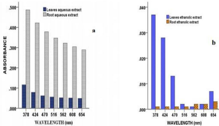
Figure 5. UV-Visible spectrophotometric profile of 0.15g/ml aqueous (a) and ethanolic (b) extracts of Petiveria alliacea leaves and root
