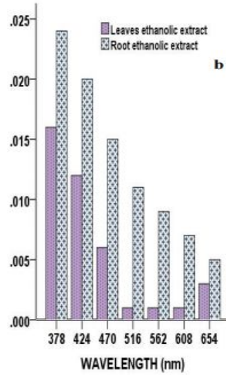
Figure 1:- UV-Visible spectrophotometric profile of 0.01g/ml aqueous (a) and ethanolic (b) extracts of Petiveriaalliacea leaves and root
