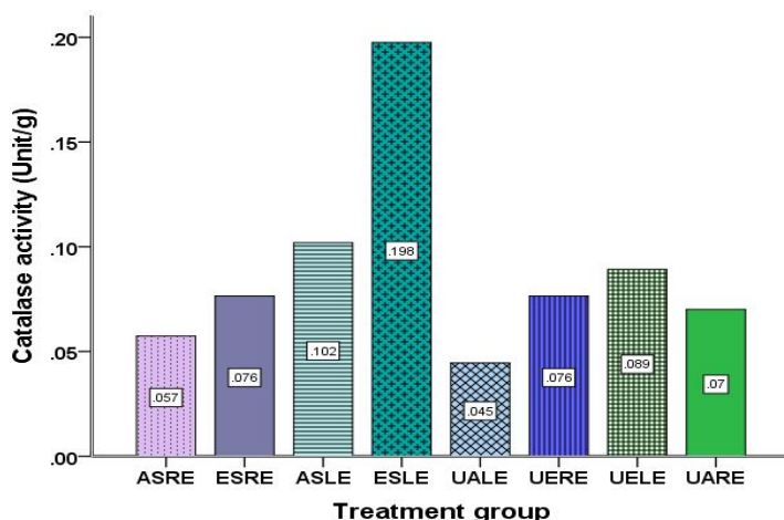
Figure 9. Catalase activity (unit/g) of soaked and unsoaked aqueous and ethanolic extracts Petiveria alliacea leaves and root
