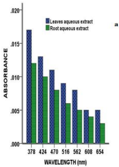
Figure 1:- UV-Visible spectrophotometric profile of 0.01g/ml aqueous (a) and ethanolic (b) extracts of Petiveriaalliacea leaves and root
