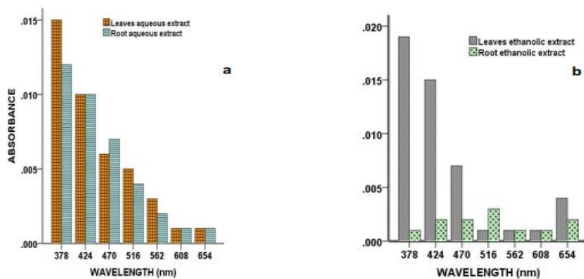
Figure 4:- UV-Visible spectrophotometric profile of 0.1g/ml aqueous (a) and ethanolic (b) extracts of Petiveria alliacea leaves and root
