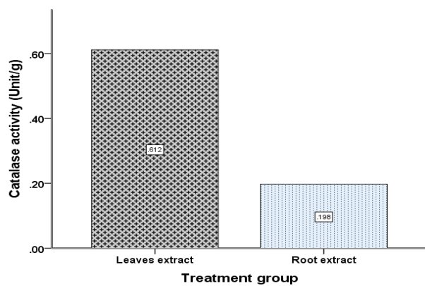
Figure 8. Catalase activity (unit/g) of phosphate buffer Petiveria alliacea leaf and root extract
