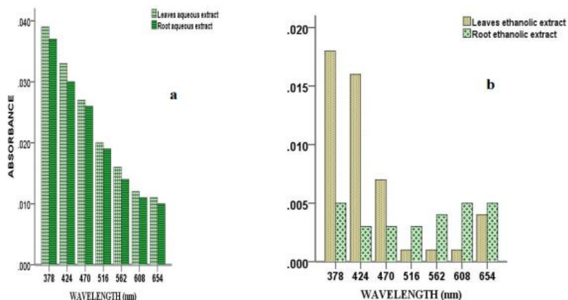
Figure 3:- UV-Visible spectrophotometric profile of 0.075g/ml aqueous (a) and ethanolic (b) extracts of Petiveria alliacea leaves and root
