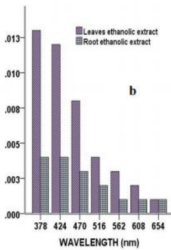
Figure 2:- UV-Visible spectrophotometric profile of 0.025g/ml aqueous (a) and ethanolic (b) extracts of Petiveriaalliacea leaves and root
