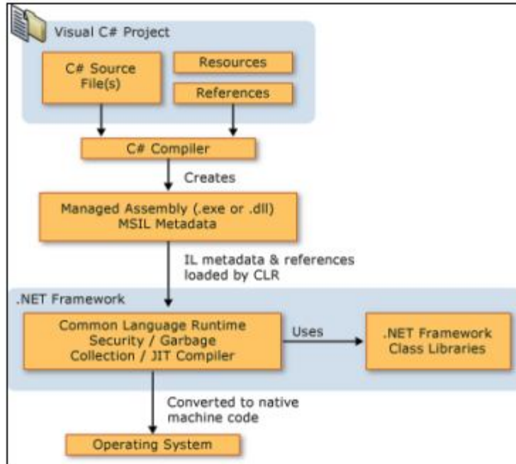
Fig. 1: .Net architecture [9]
