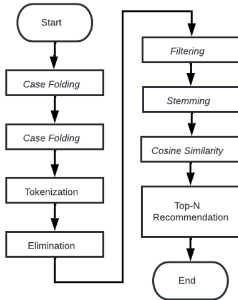
Figure 3. Flowchart Content-Based Filtering
