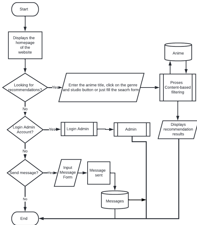
Figure 2: Flowchart of Home Page
