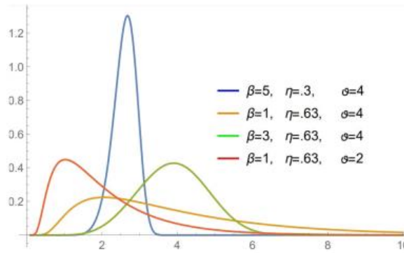
Figure 2. Weibull- IE -loglogistic distribution pdfs for different parameter values.
