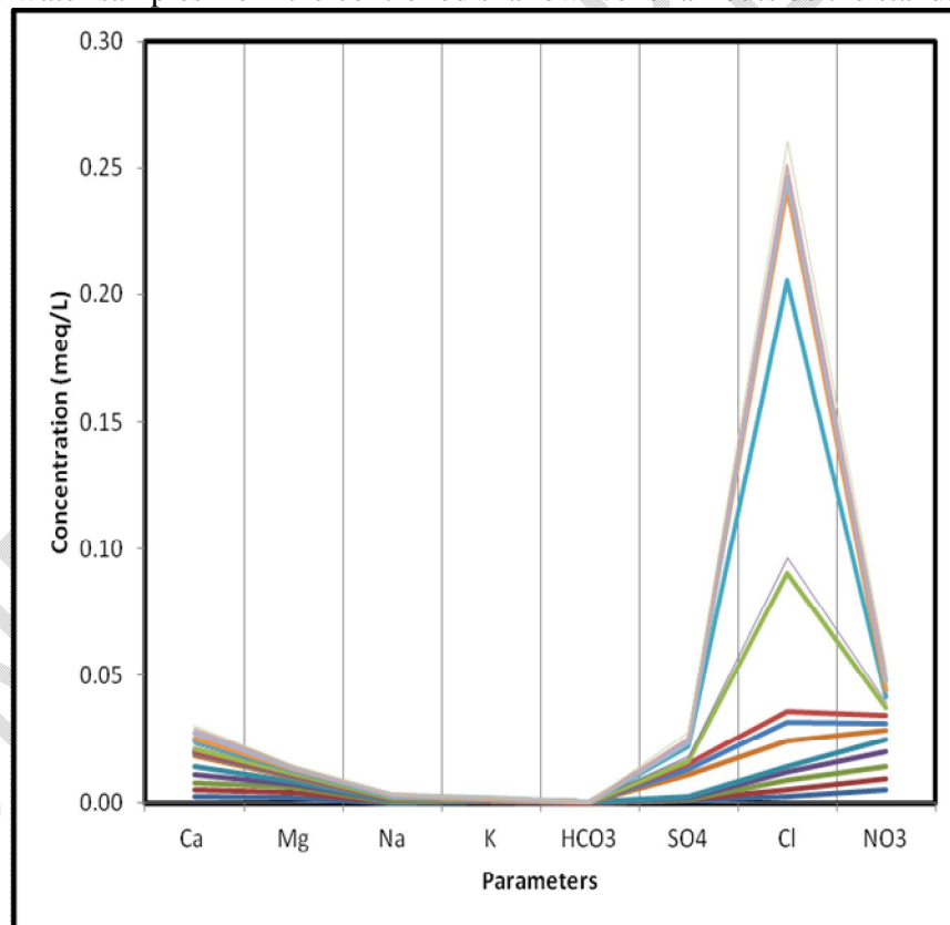
Fig. 4. Schoeller Diagram
