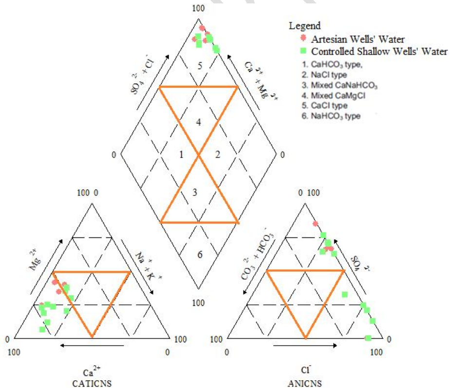
Fig. 3. Piper Diagram
