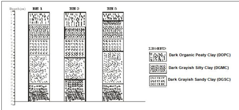
Figure 2: Representative Stratolog of Study Area
