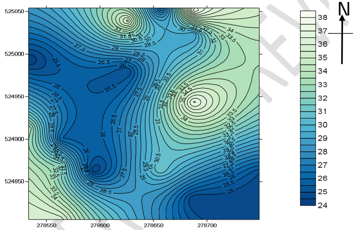
Figure 3: Liquid Limit
