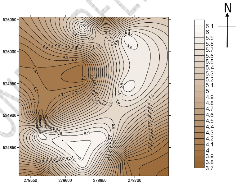
Figure 5: Angle of Internal friction
