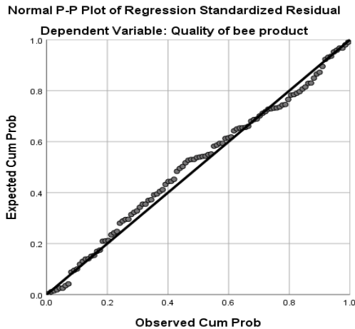
Figure 3; Linearity Test
