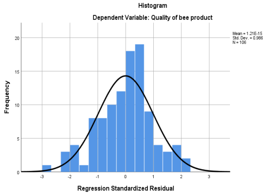
Figure 2; Normality Test
