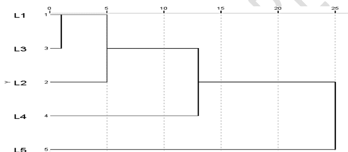
Figure 4: Dendrogram using average Linkage of the five landraces of molokhia based on the studied traits, rescaled distance cluster combine.
