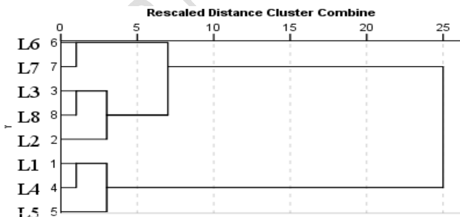
Figure 2: Dendrogram using the average Linkage of the eight landraces of okra based on the studied traits, over both seasons, rescaled distance cluster combines.
