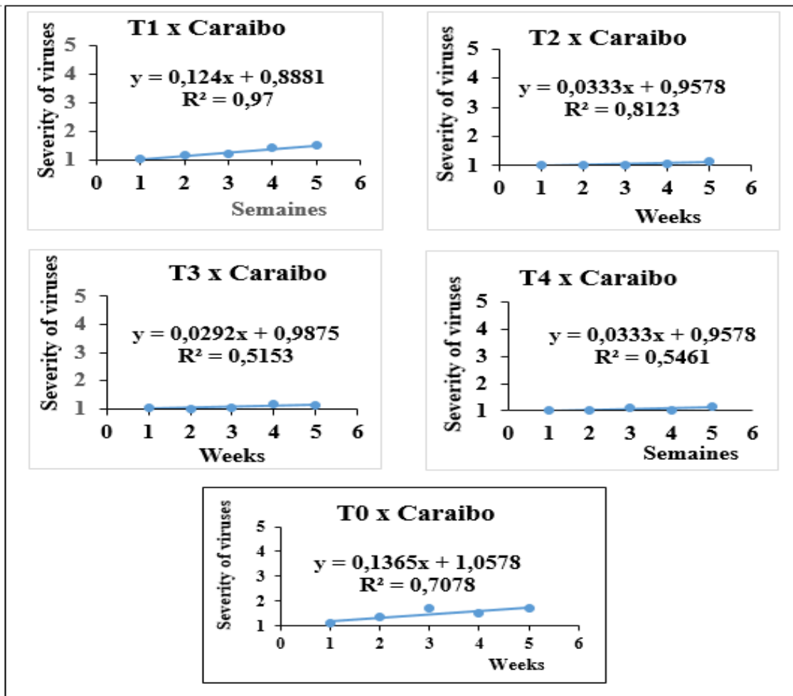
Figure 3: Linear model describing the evolution of virus severities under Caraïbo under different fertilization conditions
