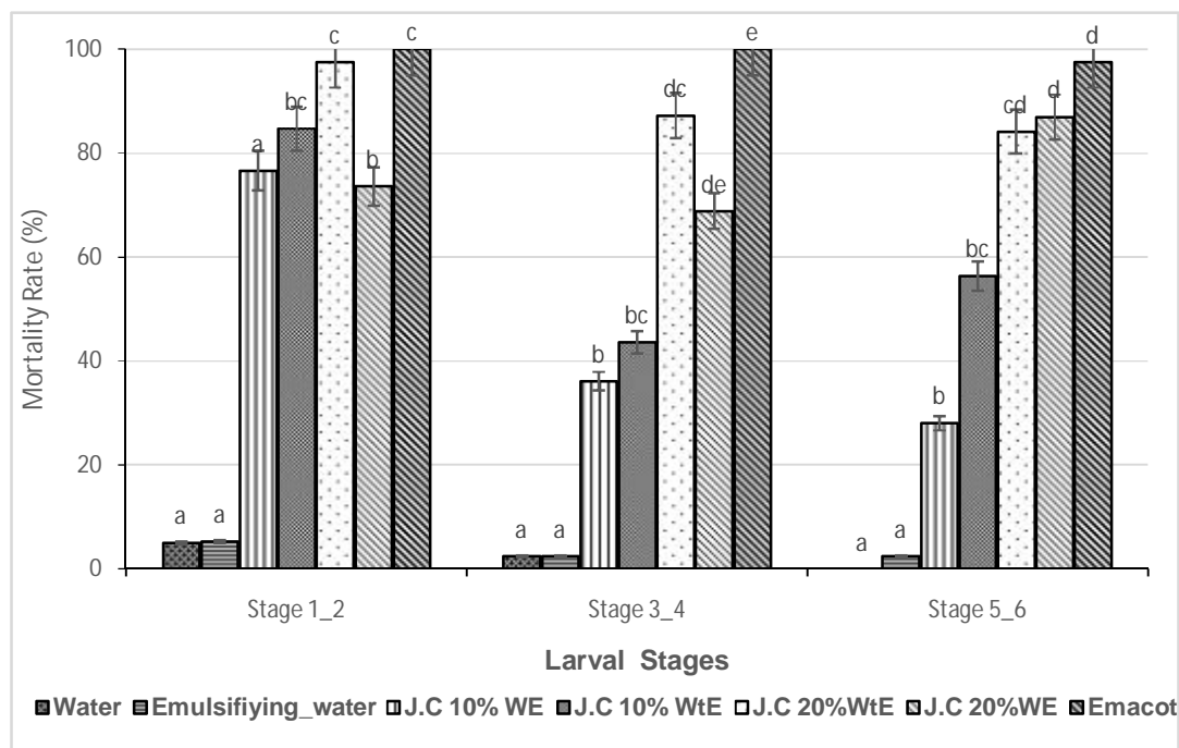
Figure 2: Mortality rate of larvae of different larval stages of S. frugiperda subjected to different formulations based on jatropha oil after 48 hours. The significant differences between the treatments are indicated by different letters (Tukey's test at the 5% threshold). J.C : J. curcas ; WtE : without emulsifier; WE : with emulsifier.
