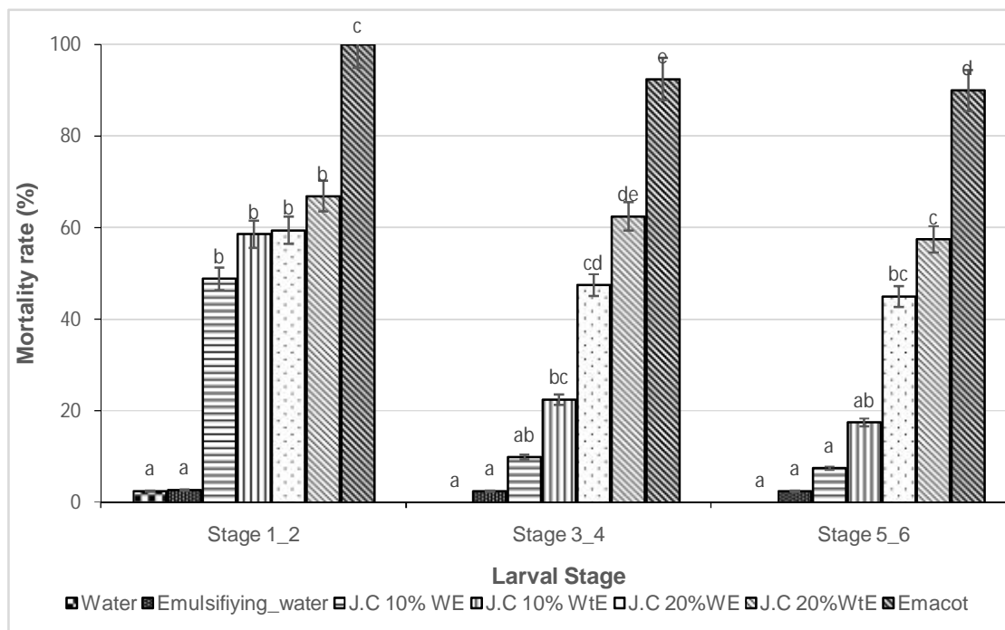
Figure 1: Mortality rate of larvae of different larval stages of S. frugiperda subjected to different formulations based on jatropha oil after 24 hours. The significant differences between the treatments are indicated by different letters (Tukey's test at the 5% threshold). J.C : J. curcas ; WtE : without emulsifier; WE : with emulsifier.
