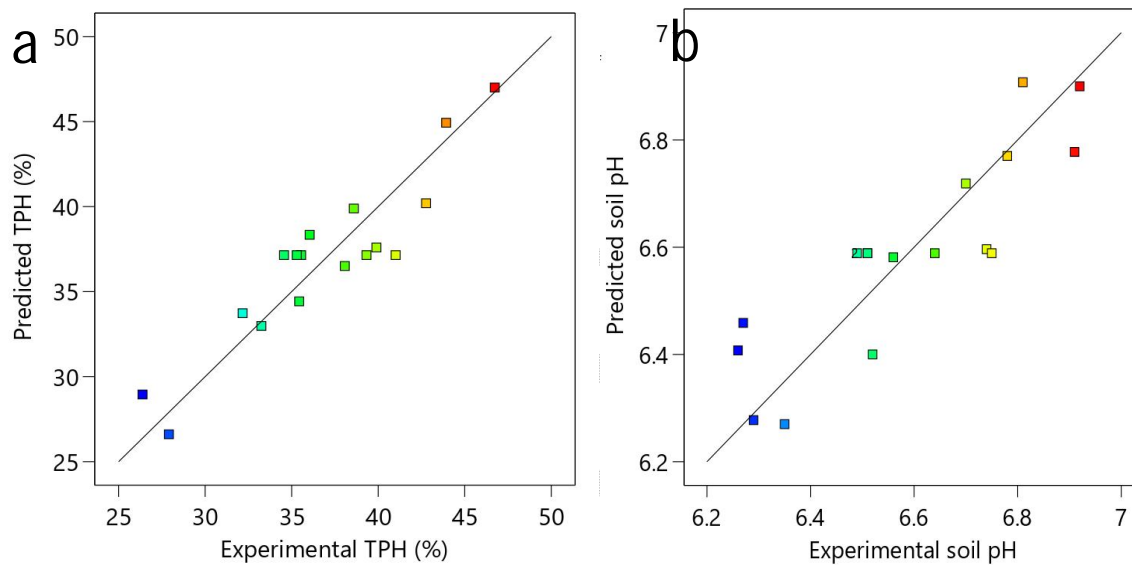
Figure 10: The relationship between experimental and predicted values of %TPH removal and soil pH.
