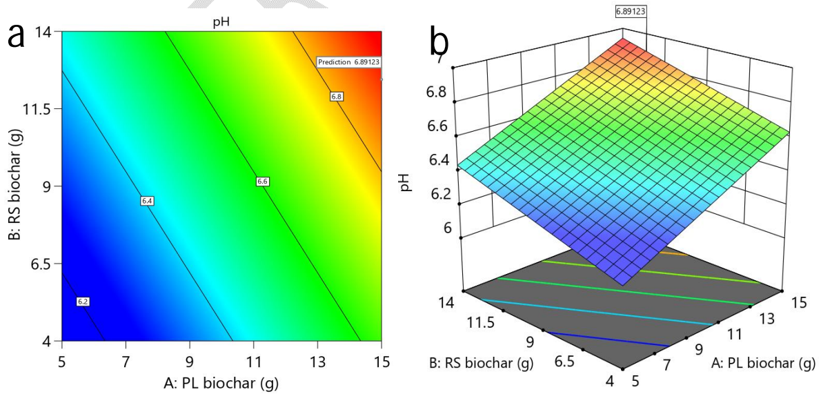
Figure 9: 2D contour and 3D surface plots for optimal conditions for soil pH effect.
