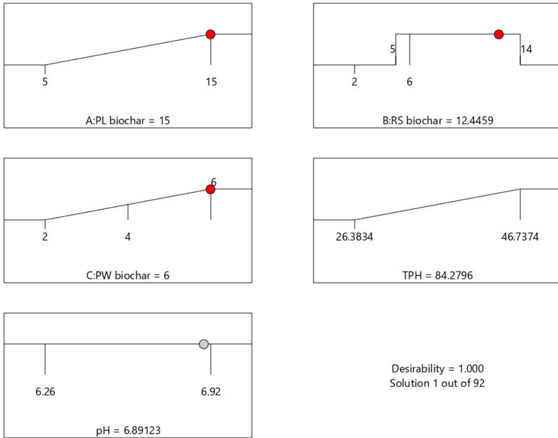
Figure 7: Ramp plot of optimal conditions for soil pH on TPH degradation.
