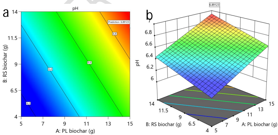
Figure 9. 2D contour and 3D surface plots for optimal conditions for soil pH effect.
