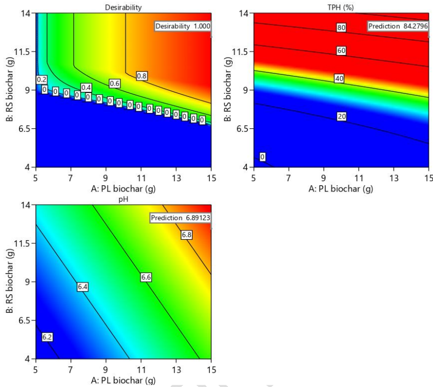
Figure 8. Desirability plots for optimization of soil pH.
