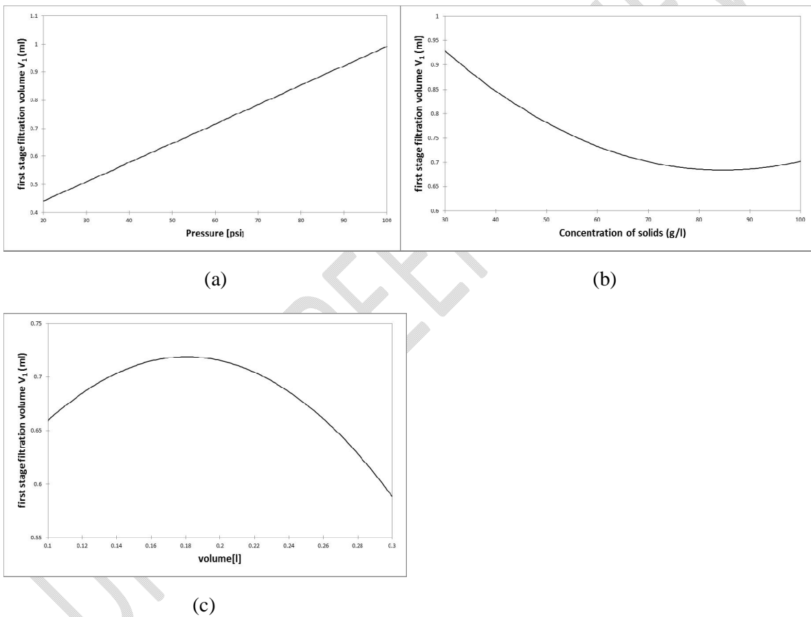
Figure 2: First stage filtration volume V_1 against (a) pressure (psi) (b) Concentration of solids (g/l) (c) Volume of slurry (litres)
