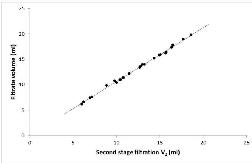
Figure 4: Relationship between filtrate volume and Second stage filtration V_2
